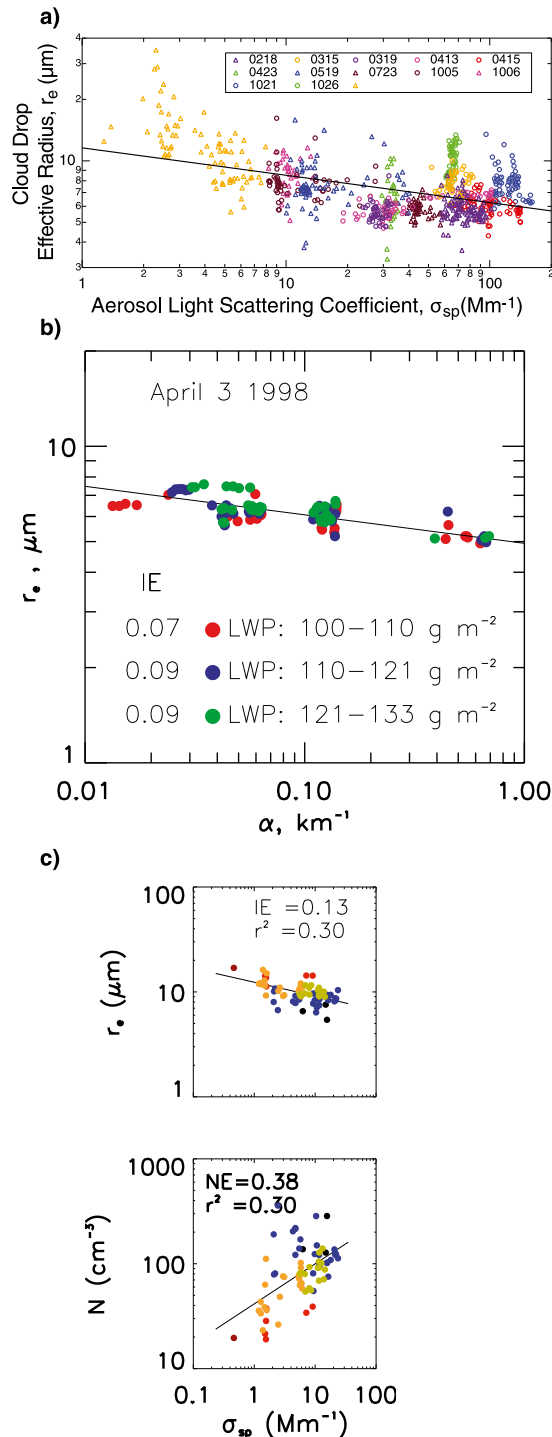
FIG. 22-1. First surface remote sensing demonstrations of the influence of the aerosol on cloud microphysical properties at ARM sites: (a) drop effective radius r_e as a function of surface aerosol light scattering \sigma_{\text{sp}} at SGP (after Kim et al. 2003), (b) r_e as a function of subcloud aerosol extinction \alpha derived from the Raman lidar at SGP (after Feingold et al. 2003), and (c) r_e and drop concentration N as a function of surface \sigma_{\text{sp}} at NSA (after Garrett et al. 2004). See text and original articles for further details on the r_e and N retrievals.
