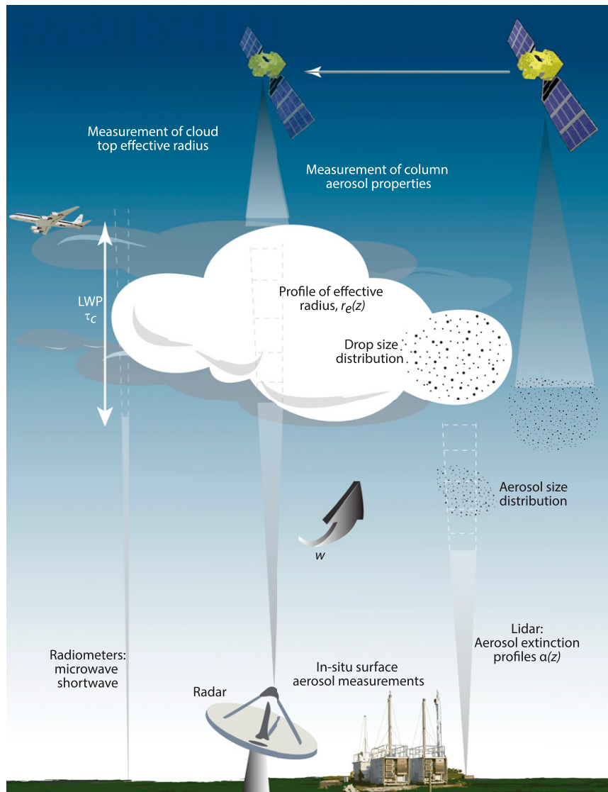
FIG. 22-2. Schematic contrasting the surface- and satellite-based remote sensing approaches to measurement of aerosol–cloud interactions. Some of the key surface instrumentation is also identified. Surface remote sensing has the advantage of being able to identify the aerosol entering the clouds from below while satellite remote sensing must contend with measuring column-integrated aerosol in cloud-free columns and cloud microphysics in adjacent cloudy columns. Satellite data have the advantage of global coverage while surface remote sensing is limited to a few sites, although at high temporal resolution.
