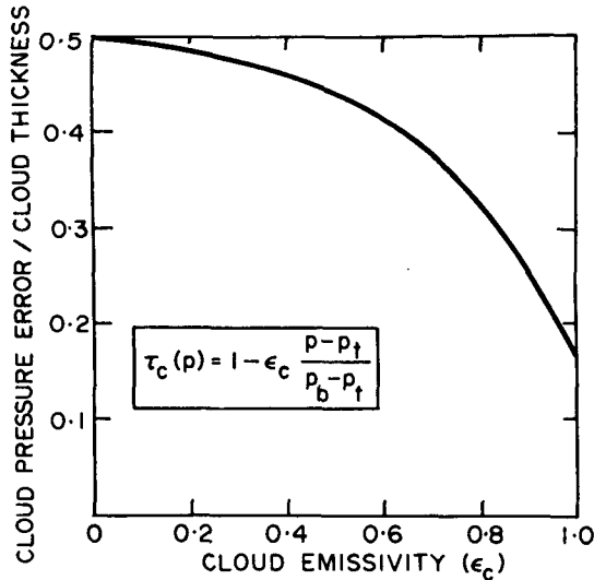
FIG. 1. Error due to infinitesimal cloud thickness assumption as a function of cloud opacity.
