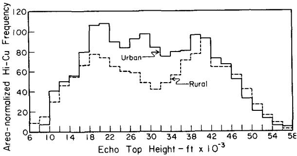
FIG. 4. Area-normalized height distributions of urban and rural hi-cu.
