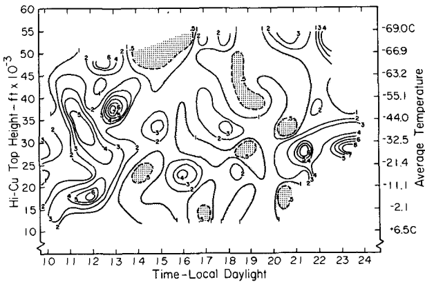
FIG. 5. Joint time-height distribution of urban hi-cu frequencies relative to rural values.
