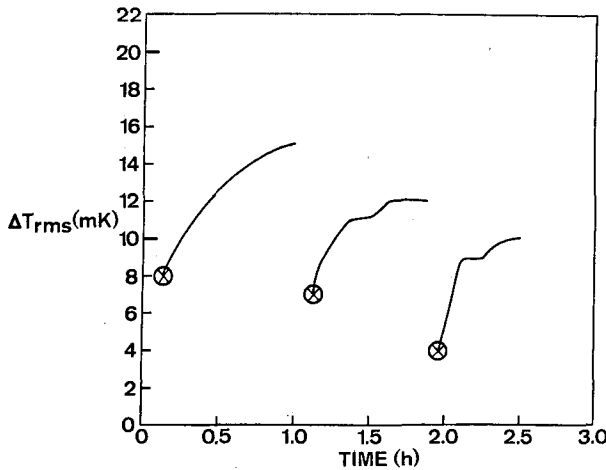
FIG. 1. Strip chart record of rms temperature difference fluctuations versus time. ⊗'s designate washing of the wires.
