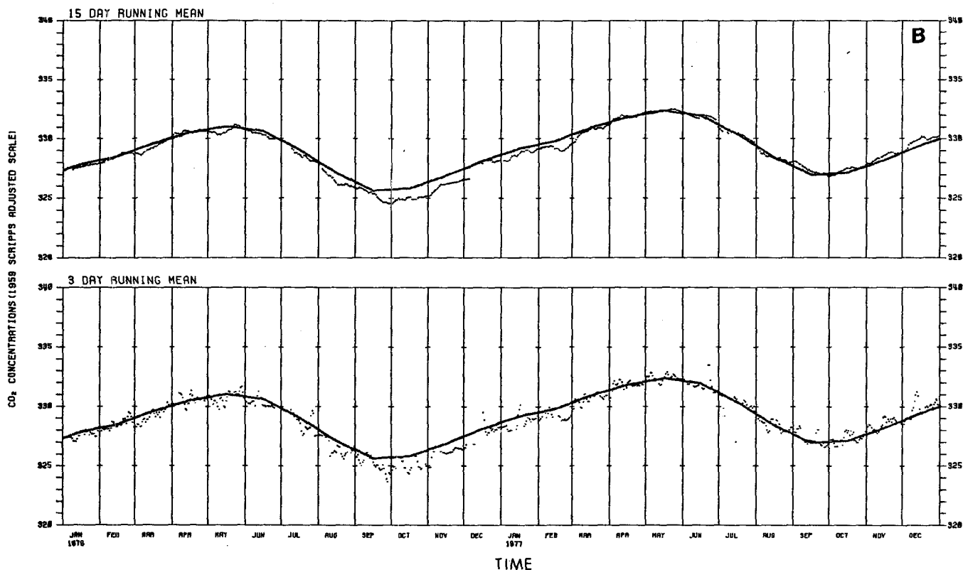
FIG. 3. Fifteen-day and three-day running means of CO 2 at MLO. Full lines show seven-year monthly means with trend incorporated.
