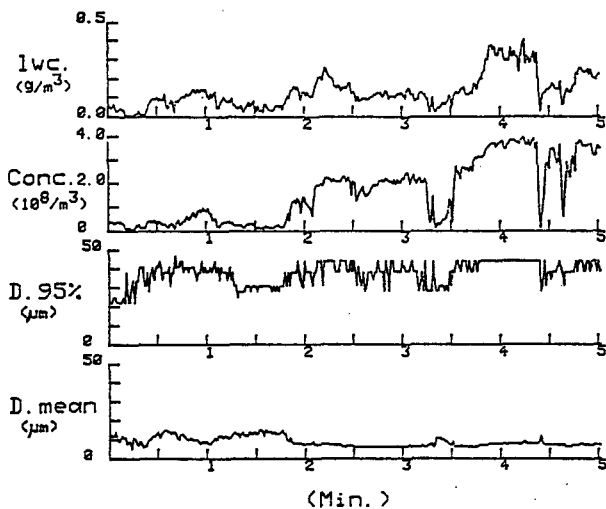
FIG. 3b. Horizontal leg for the cloud (280 m thick) observed on 13 June at 860 m height (20 m below cloud top).
