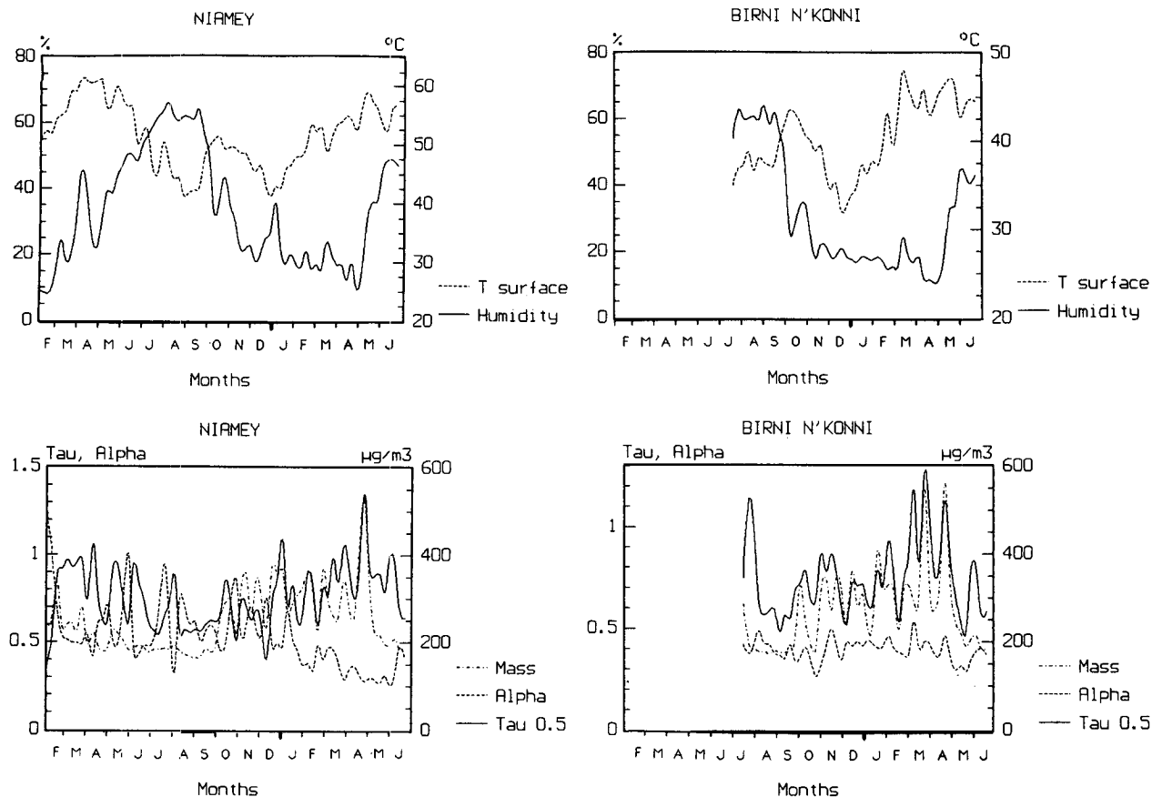
FIG. 3. (a)–(g): Weekly mean values of ground skin temperature T_s , relative humidity H , mass concentration (mass), Ångström wavelength exponent \alpha (alpha), and aerosol optical thickness at 500 nm ( \tau_{0.5} ) versus months (from February 1986 to June 1987) at sites.
