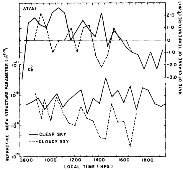
FIG. 3. Temporal variations of C_n^2 and \Delta T/\Delta t on a typical clear-sky day and cloudy-sky day.
