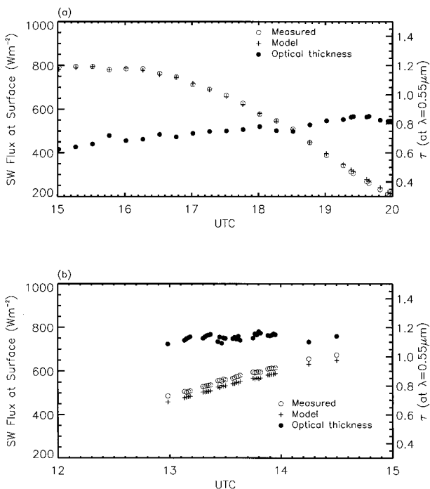
FIG. 3. Comparison between measured (open circles) and calculated (+ signs) DSWI for (a) 27 Aug 1995 and (b) 1 Sep 1995 over Cuiaba as a function of UTC time. Also shown in solid circles is the measured aerosol optical thickness at 0.55 \mu\text{m} .
