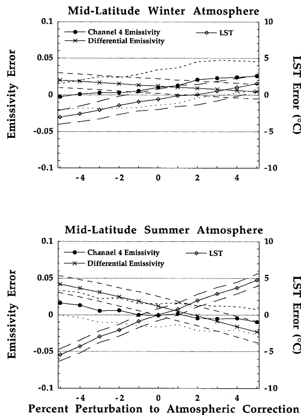
FIG. 1. Results of retrieval sensitivity experiments. Top panel is for midlatitude winter atmosphere; bottom panel is for midlatitude summer atmosphere.
