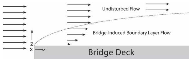
FIG. 2. Bridge-induced boundary layer and coordinates used in convective parameterization.
