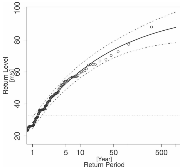
FIG. 2. Return-level plot for storms passing within 495 km of Lake Shelby. The curve represents the extreme value model and it asymptotically approaches finite return levels because the \xi parameter is less than zero. Parameter estimates are made using the maximum likelihood approach. The thin lines are the 95% confidence limits. The return level is the expected maximum hurricane intensity ( \text{m s}^{-1} ) over r years. The points are the empirically estimated return levels for each hurricane occurring within the region.
