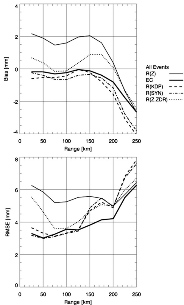
FIG. 12. (top) Mean bias and (bottom) RMS error of different radar estimates as a function of range (43 rain events, 179 h of observation).
