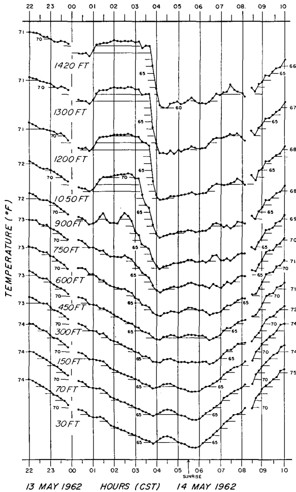
FIG. 2. Time variation of temperature at the 12 levels of the Cedar Hill tower from 2200 CST, 13 May to 1000 CST, 14 May 1962.
