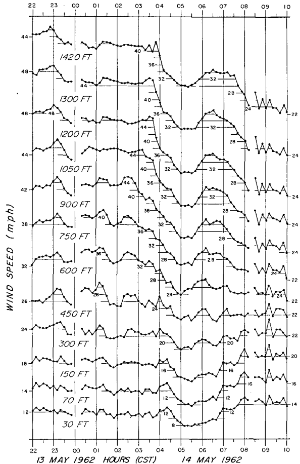
FIG. 3. Time variation of wind speed at the 12 levels of the Cedar Hill tower from 2200 CST, 13 May to 1000 CST, 14 May 1962.
