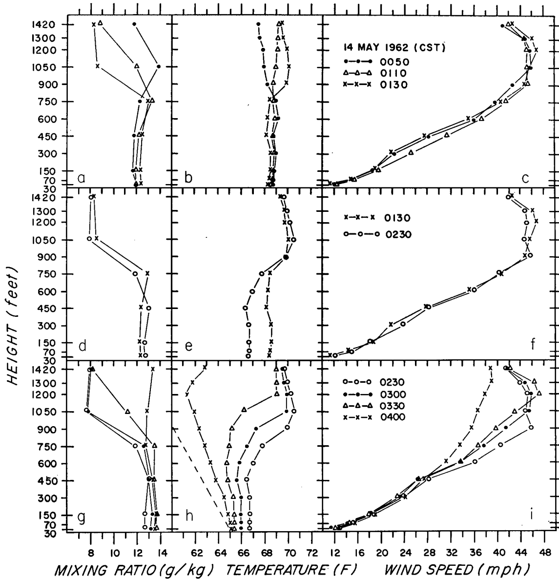
FIG. 5. Vertical profiles of mixing ratio, temperature, and wind speed observed at the Cedar Hill tower during the early morning hours of 14 May 1962. Dashed line in Fig. 5h represents dry adiabat.
