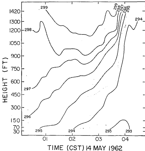
FIG. 6. Time and height variations of potential temperature and of the upper and lower boundaries of temperature inversions observed at the Cedar Hill tower during the early morning hours of 14 May 1962. Shaded areas represent temperature inversions.
