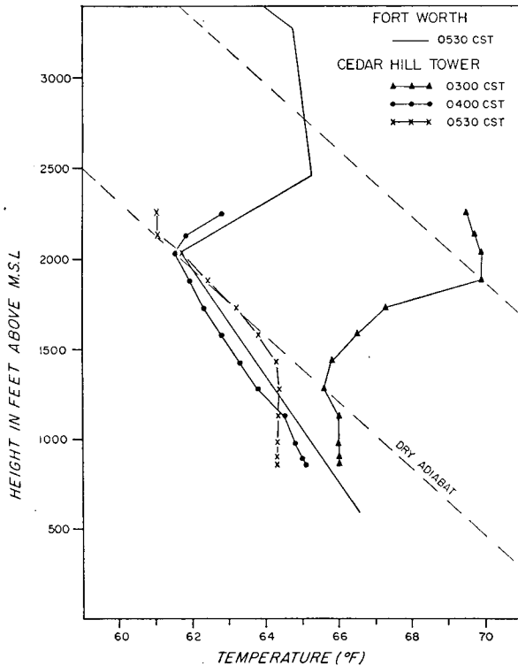
Fig. 8. Fort Worth temperature sounding for 0530 CST and Cedar Hill tower temperature profiles for 0300, 0400, and 0530 CST, 14 May 1962.
