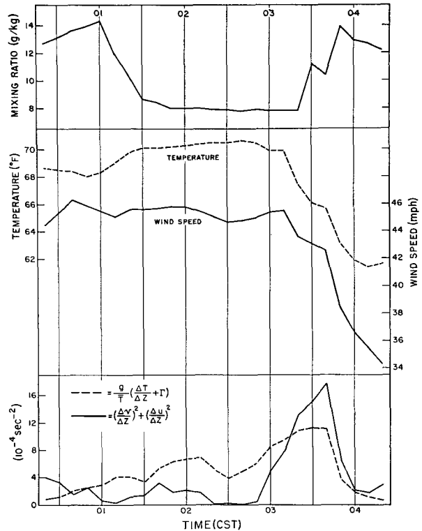
FIG. 7. Time variations of the numerator and denominator of the Richardson number, mixing ratio, temperature, and wind speed at 1050 ft of the Cedar Hill tower during the early morning hours of 14 May 1962.
