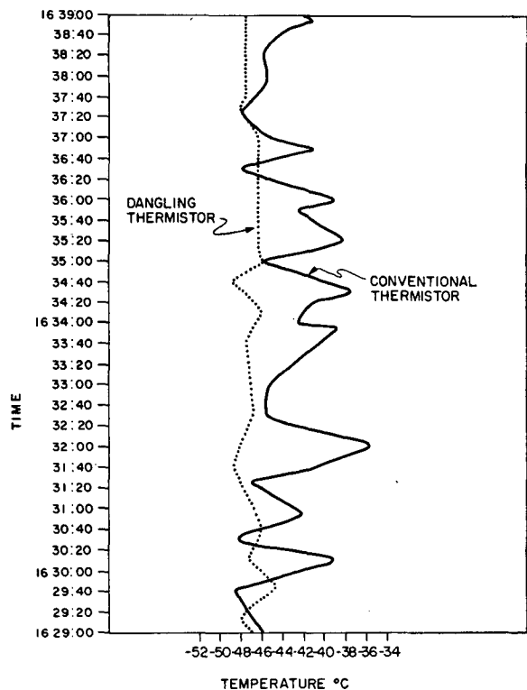
FIG. 7. A comparison of temperature traces from a regularly positioned and a dangling thermistor taken by one radiosonde on 3 June 1964 at 30 mb pressure altitude. The humidity circuit was suitably adapted to a temperature circuit for a dangling thermistor. (Time is in minutes and seconds.)
