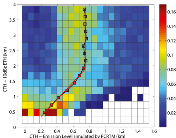
FIG. 3. The 2D histogram of the distance between CTH and the EEL computed by PCRTM (abscissa) vs the distance between CTH and ETH_{10\text{dBZ}} (ordinate). The figure is normalized for each CTH – ETH_{10\text{dBZ}} interval. The black squares show the expected distance between CTH and EEL from such probability distributions. The red line is the regressed results.
