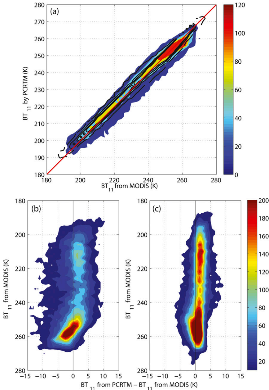
FIG. 5. (a) The 2D histogram of the numbers of occurrences of the 11- \mu\text{m} brightness temperature ( BT_{11} ) measured by MODIS (abscissa) and simulated using PCRTM with CloudSat cloud water profiles and temperature and humidity profiles as described in the text (ordinate). The red line with a slope of 1:1 is plotted as a reference. Color-filled contours are results assuming CTT equal to the ambient air temperature. The black contours are the result from updated estimation of CTT described in section 4. The difference between simulated BT_{11} and MODIS measurements with respect to MODIS BT_{11} (b) with and (c) without non-blackbody correction. The same color contours are used in (b) and (c).
