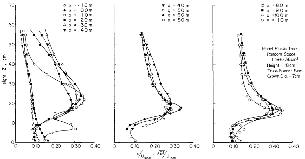
FIG. 7. Longitudinal turbulent intensity for model forest canopy.
