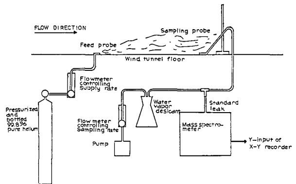
FIG. 5. Continuous point source feed and sampling systems.
