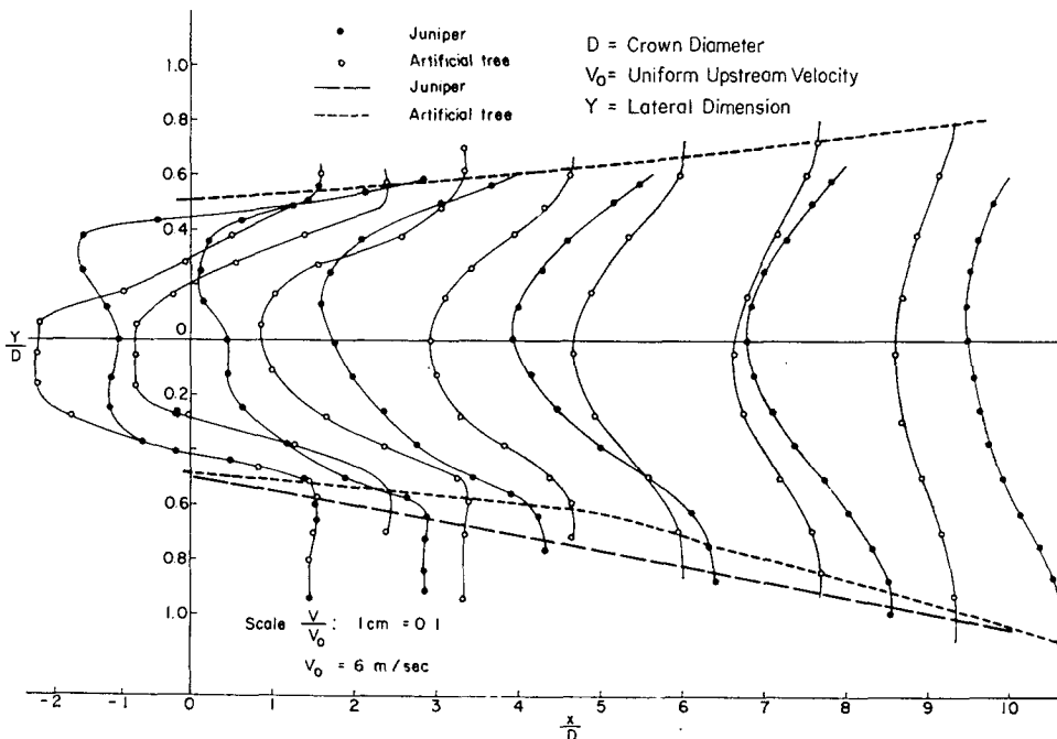
FIG. 2. Wake characteristics of live and model trees.
