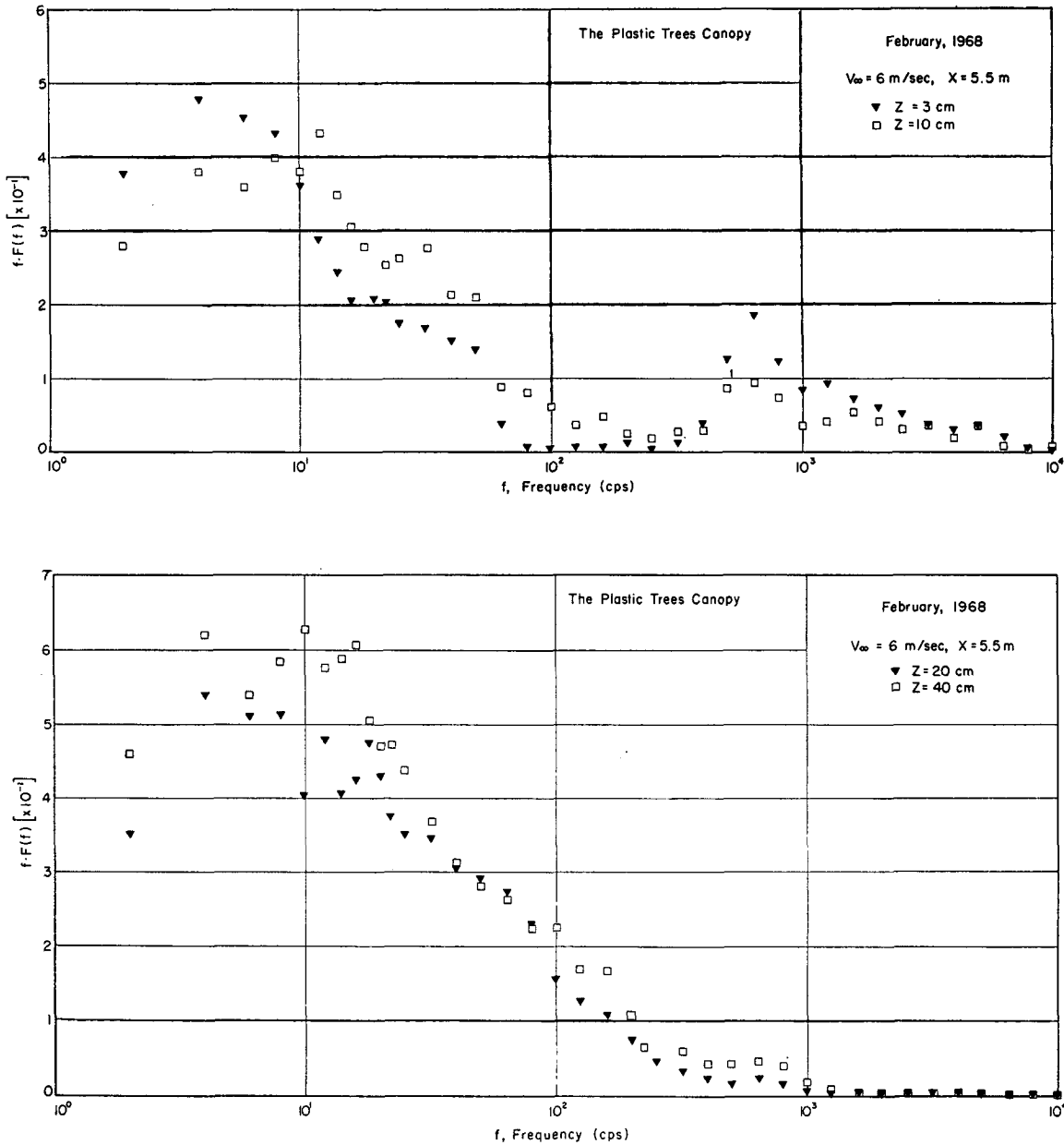
FIG. 9. Turbulent energy distributions in model forest canopy for various heights above the ground.
