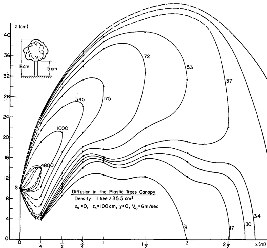
FIG. 10. Diffusion plume at model forest entrance region.
