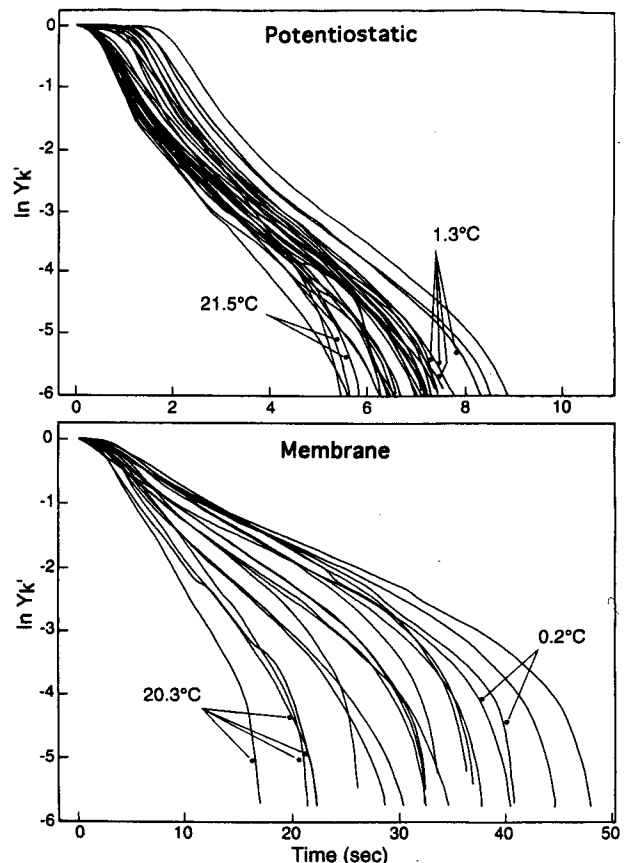
FIG. 1. The response of potentiostatic (POS) and membrane (MOS) oxygen sensors illustrated as \ln Y'_k versus time, where Y'_k = (Y_f - Y_t)/(Y_f - Y_i) . Here Y_f was chosen as 99% of the final value to illustrate the entire response. Note that the response of the MOS is about five times slower than the POS.
