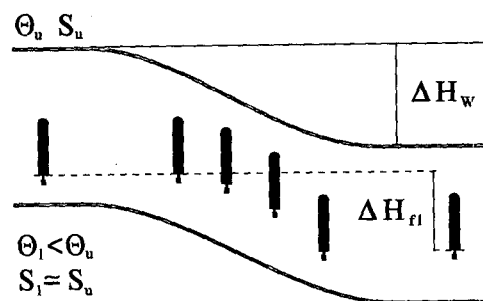
FIG. 2. Schematic of linked relative motion of float and corresponding waterbody. The float drifts within an assumed waterbody exhibiting a small salinity gradient and a negative temperature gradient \partial T/\partial p . If this waterbody descends, the float tries to follow. However, since it is not as compressible as the surrounding water it gains buoyancy while sinking, ending up in warmer water than before.
