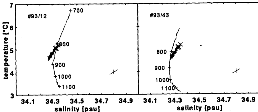
FIG. 12. The T - S diagrams of float 93 compared to CTD casts 12 and 43. CTD 12 was taken when the float was launched; 43 is a CTD farther west, taken at the beginning of the trajectory of float 70 crossing that of float 93 twice. The numbers at the curve indicate the corresponding pressure (db).
