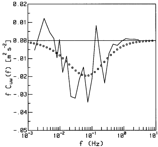
FIG. 9. The corrected (solid line) covariance spectra for the longitudinal component of the momentum flux plotted with a parameterization of this component (dotted line) reported in Kaimal et al. (1972).
