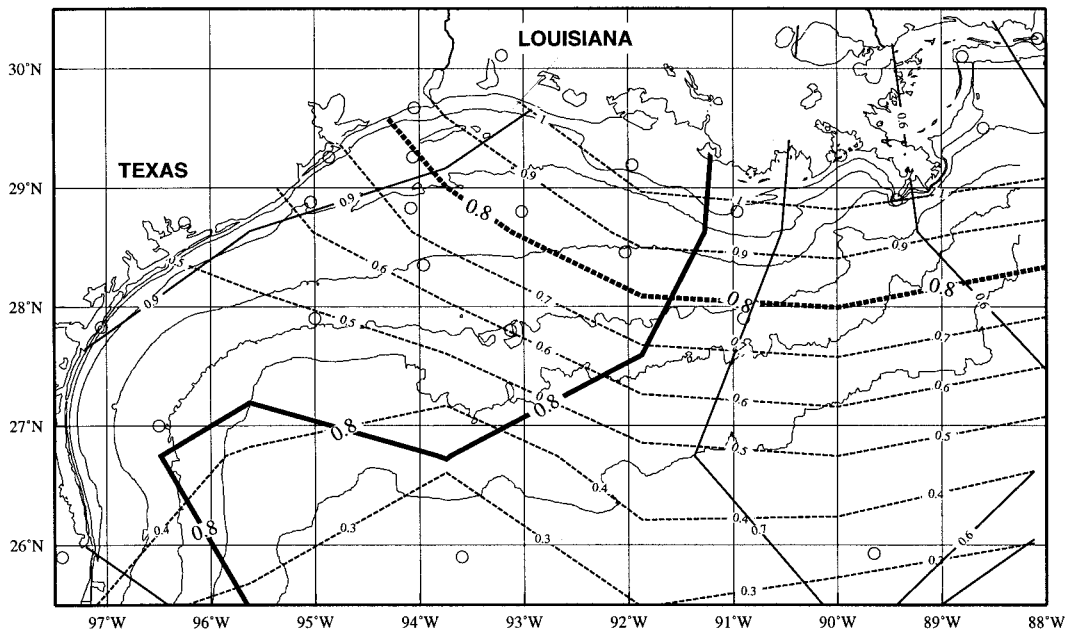
FIG. 3. Significance levels (based on Student's t-test) for differences between LATEX and NCEP wind components. Solid lines are for eastward components; dashed lines are for northward components.
