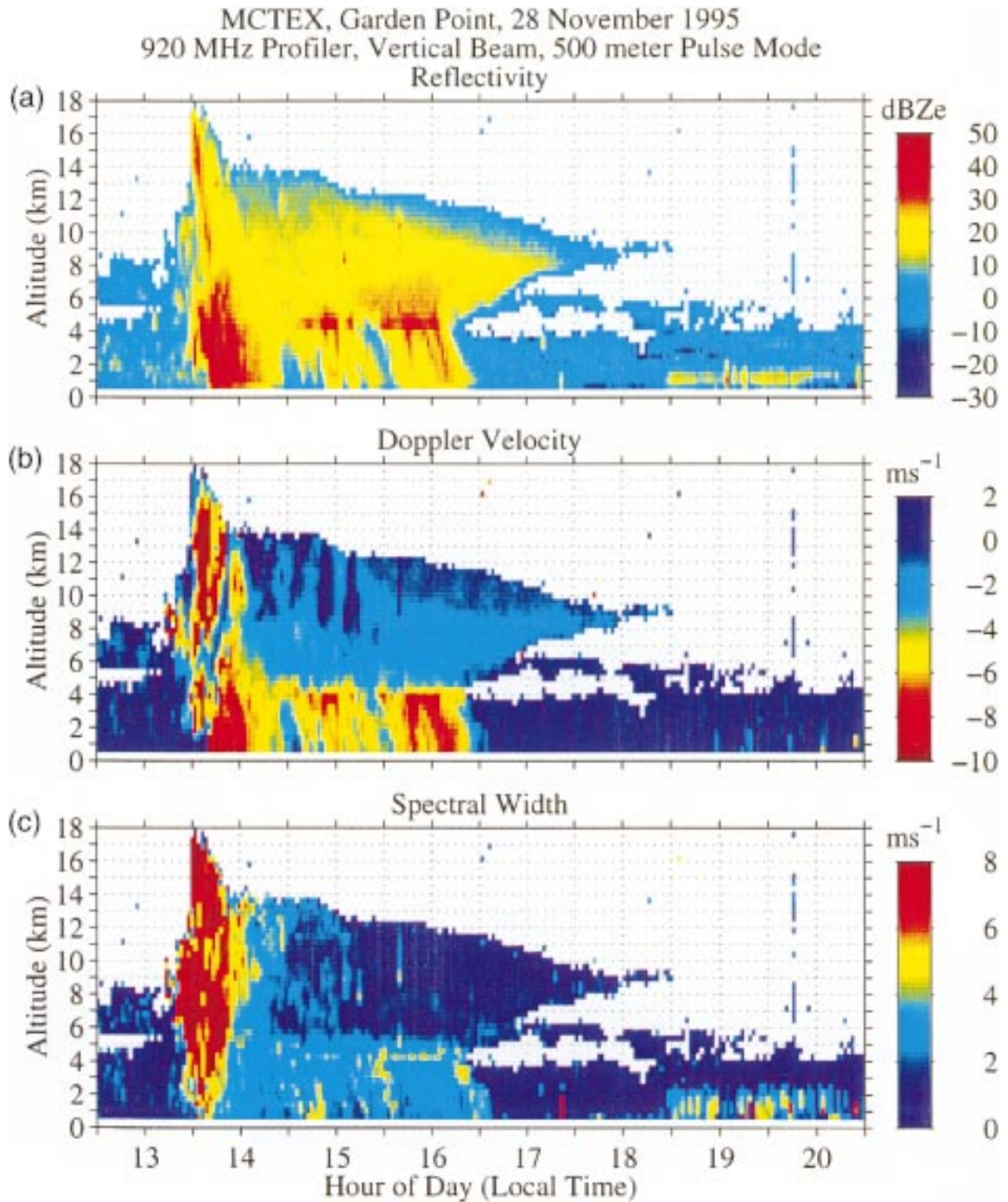
FIG. 6. Time–height sections of (a) equivalent reflectivity, (b) Doppler velocity, and (c) spectral width for observations made by the 920-MHz profiler at Garden Point on 28 November 1995.
