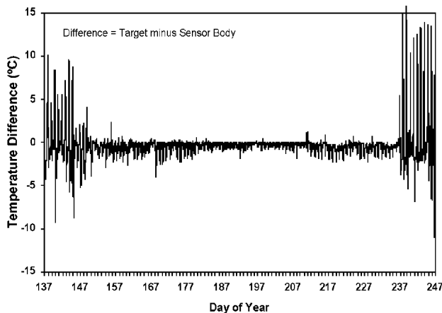
FIG. 4. Time series plot of the difference ( ^{\circ}\text{C} ) between the IRT target and sensor body temperatures for 17 May–4 Sep (days 137–247) 2001.
