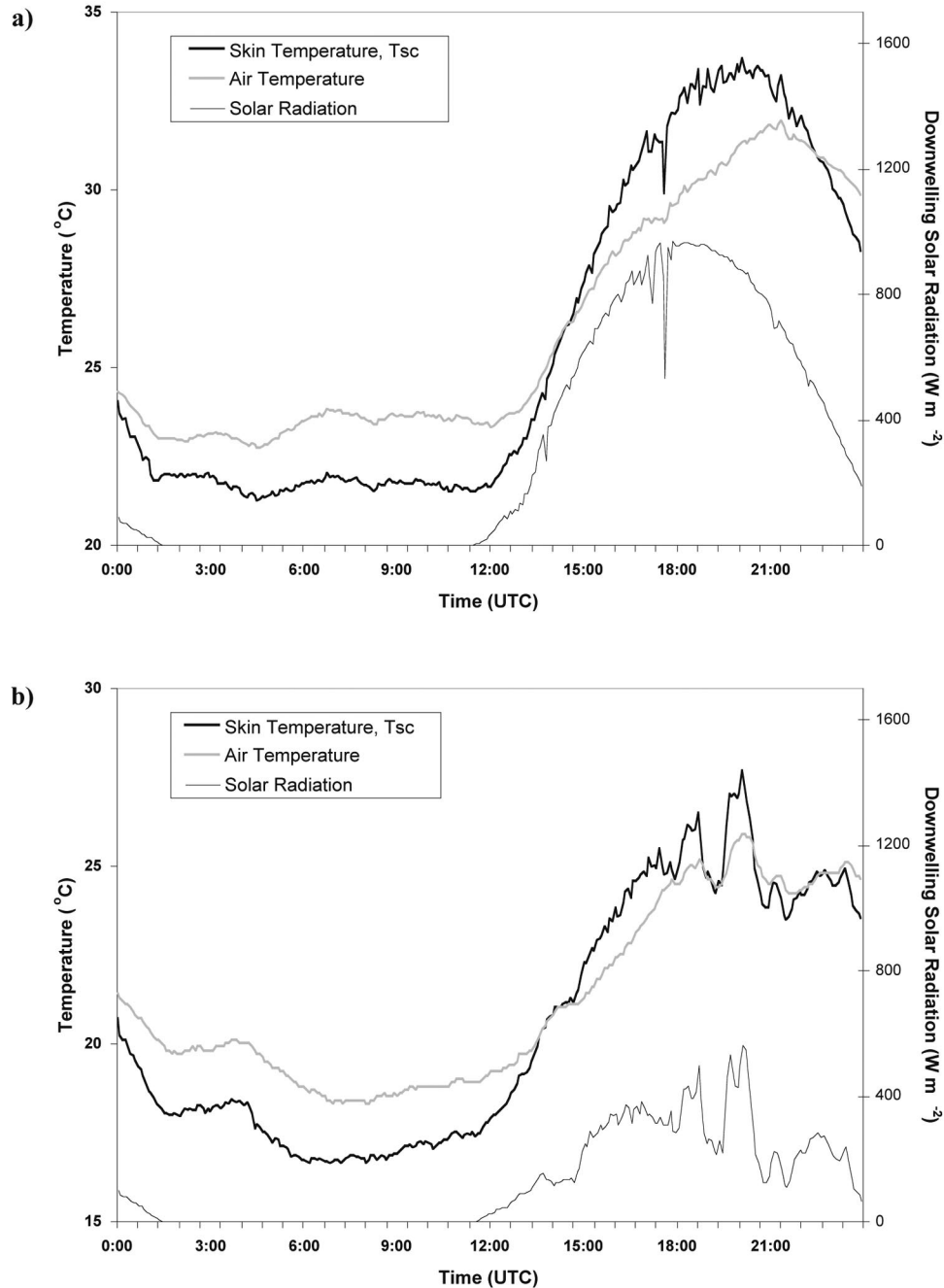
FIG. 2. Time series plot of the T_{sc} ( ^{\circ}\text{C} ), air temperature ( ^{\circ}\text{C} ), and downwelling solar radiation ( \text{W m}^{-2} ) at the Mesonet site near Marena, OK, on (a) 11 May and (b) 16 May 2000.
