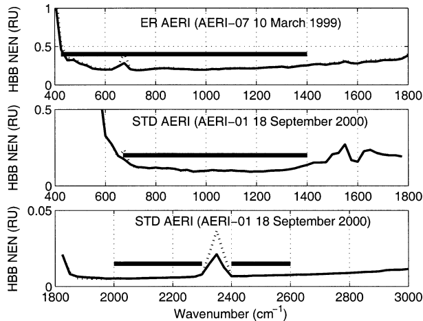
FIG. 12. The noise specification on the hot blackbody reference view for the longwave band of (top) an ER-AERI, (middle) the longwave band of a standard AERI, and (bottom) the shortwave band of any AERI, shown with horizontal solid lines. The two curves (solid and dotted) are the hot blackbody noise estimate from the two real-time AERI noise products. The two noise estimates agree so well that the curves fall directly on top of each other. [Radiance units: \text{RU} = \text{mW} (\text{m}^2 \text{sr cm}^{-1})^{-1} .]
