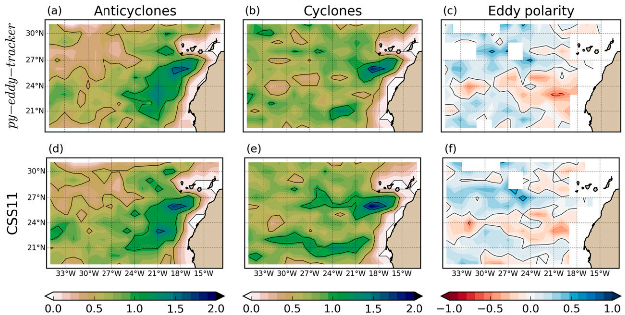
FIG. 2. Contour plots of Canary Eddy Corridor mean eddy counts per 1^\circ square per year and eddy polarity from (top) py-eddy-tracker and (bottom) CSS11 , and (left) anticyclone counts ( n_a ), (middle) cyclone counts ( n_c ), and (right) polarity [(n_c - n_a)/(n_c + n_a)] . Regions in the polarity maps where either n_c < 0.25 or n_a < 0.25 are masked.
