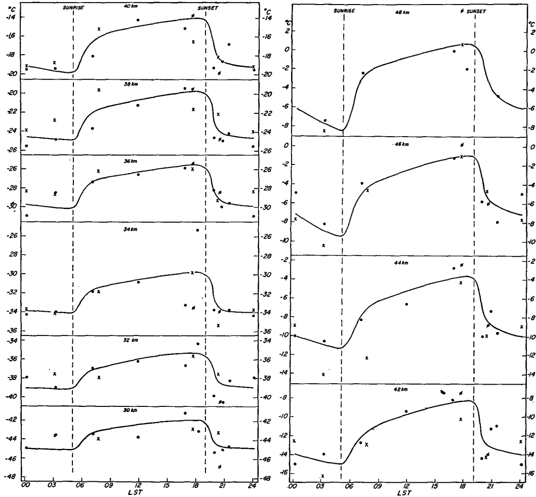
FIG. 2. Analyses of mean rocketsonde temperatures for 4-km layers. Observations taken during a 39-hr period have been compressed into a 24-hr interval. Dots, data obtained between 1600 EST 8 September and 1600 EST 9 September 1965; solidus through dots, ARCAS reports; crosses, data obtained between 1600 EST 9 September and 0800 EST 10 September.
