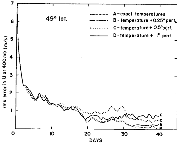
FIG. 1. The rms error in zonal wind ( m\ sec^{-1} ) at 400 mb at 49^\circ latitude, in cases where temperatures with random error perturbations of 0, 0.25, 0.5 and 1C are inserted every 12 hr at all grid points.
