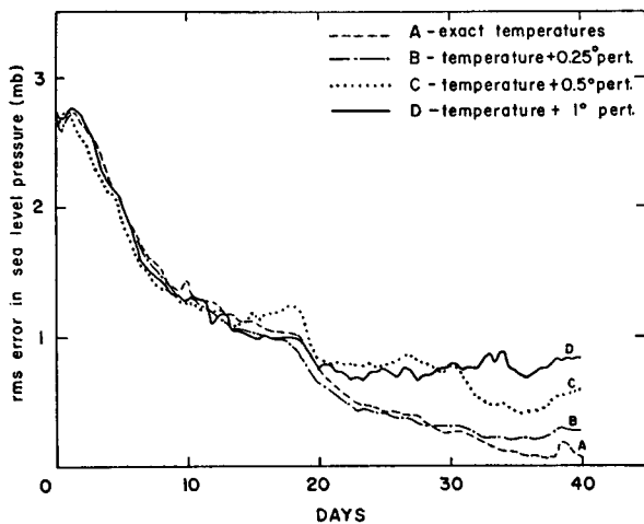
FIG. 3. The rms error in sea level pressure anomaly (mb) for the Northern Hemisphere, in cases where temperature with 0, 0.25, 0.5 and 1C random error perturbations are inserted every 12 hr at all grid points.
