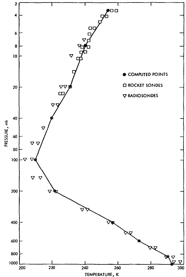
FIG. 7. Temperature profile derived from 0605 radiance data. The estimated cloud cover was less than 4% and the profile was obtained by assuming no clouds.
