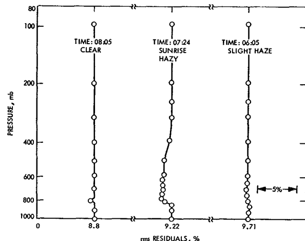
FIG. 8. Variation of residuals with assumed cloud pressure levels for 0605, 0724 and 0805 CDT radiance data.
