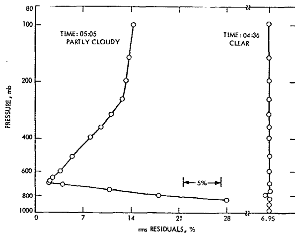
FIG. 6. Variation of residuals with assumed cloud pressure levels for 0436 and 0505 radiance data.
