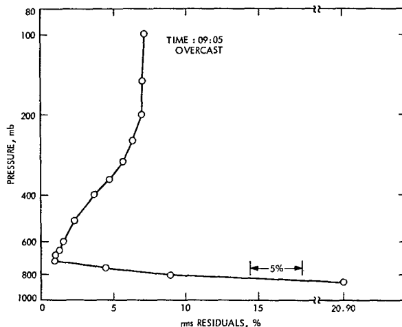
FIG. 12. Variation of residuals with assumed cloud pressure levels for 0905 CDT radiance data.
