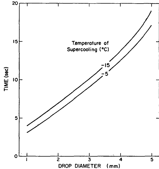
FIG. 12. Time after complete freezing for a drop to cool vs drop diameter for two values of air (supercooling) temperature.
