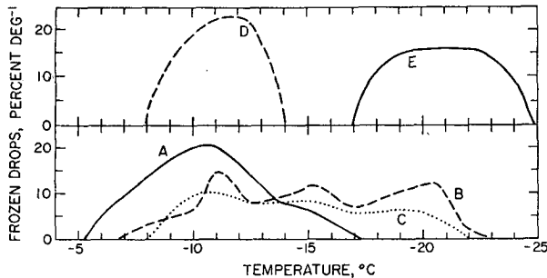
FIG. 6. Freezing temperature spectra of two soil suspensions (A, B, C: New Raymer, Colo.; D, E: Fort Collins, Colo.) filtered through different diameter pore filters: A, 0.22 \mu ; B, 0.01 \mu ; C, 0.8 and 0.01 \mu , successively; D, 0.8 \mu ; and E, 0.8 and 0.01 \mu , successively.
