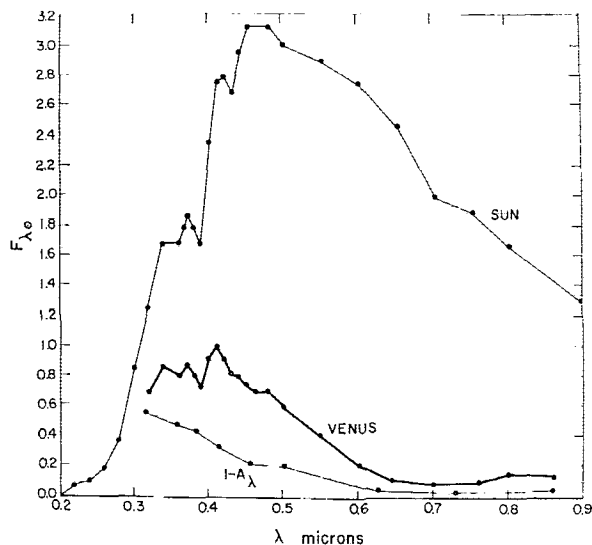
FIG. 2. Spectral distribution of the solar energy absorbed by Venus. Upper curve: solar energy distribution; bottom curve: fraction of sunlight absorbed (1 - A λ ) at each wavelength; middle curve: energy absorbed by Venus. Note that the absorbed energy is mostly in the region around 4000 Å.
