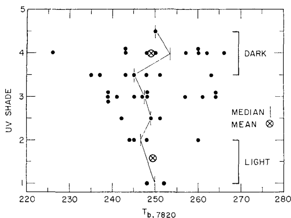
FIG. 4. Relation between UV cloud features and \text{CO}_2 rotational temperatures. Although there is no systematic variation of mean temperature with light or dark UV features, the darker features appear to show more temperature variation than the lighter ones. The scatter in the light-feature temperatures is comparable to their internal errors (3–4 K), so they may be nearly isothermal.
