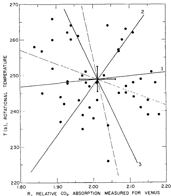
FIG. 3. Relation between CO 2 rotational temperatures and amount of absorption in the 7820 Å band. Curve 1 shows the variation to be expected if the aerosol number density varies in an atmosphere of fixed temperature-pressure profile. Curve 2 is the relation expected from temperature variations in a 75% H 2 SO 4 aerosol, as described in the text. Curve 3 is the effect of temperature alone on the equivalent widths of the CO 2 lines measured, for a fixed amount of gas. This last effect appears to be present, but is hard to see because of large, uncorrelated variations in the amount of CO 2 . The two light, unlabelled lines are the two regression lines; note that only curve 3 is contained between them. The heavy cross is centered at the means of R and T , and indicates ±1 internal standard error in each coordinate.
