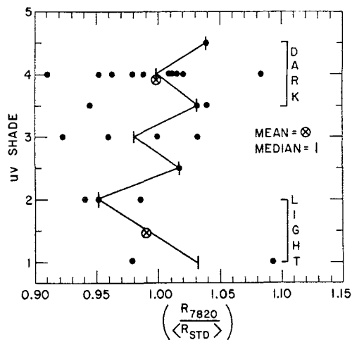
FIG. 1. Relation between the relative amount of CO 2 absorption and the relative brightness of the corresponding part of the planet in ultraviolet light. To remove the effect of daily variations in CO 2 absorption, the ratio of the amount observed in a particular area to the average for the standard slit position (parallel to the line of cusps and midway between limb and terminator), which averages over a large part of the disk, is used. The estimated brightness of each area on UV photographs runs from 1 (very bright) to 5 (very dark). The CO 2 absorptions are taken from A. Young et al. (1974) and the UV pictures were taken at the New Mexico State and Table Mountain Observatories on the same days as the infrared spectra.
