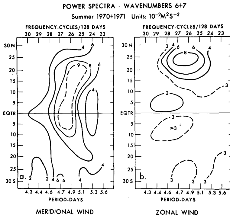
FIG. 9. As in Fig. 6 except for wavenumbers 6 and 7. Periods range from 4.3 to 5.6 days.
