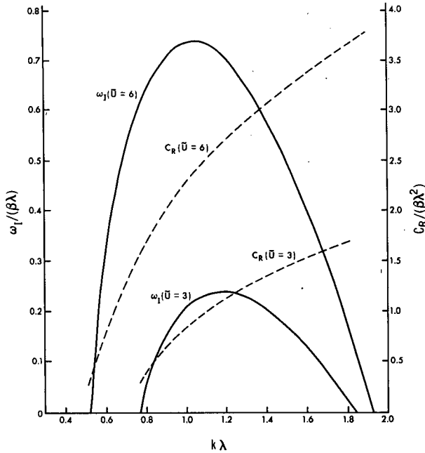
FIG. 1. Growth rates ( \omega_i ) and phase speeds ( c_R ) as a function of zonal wavenumber for the unstable mode symmetric about z = 0 on the basic state defined in (3.11), for \bar{U} = U_0/(\beta\lambda^2) = 3 and 6.
