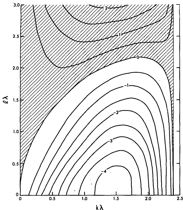
FIG. 5. m(k, l) for Eady's model, with g(z) = 1 . The region in which m > 0 is shaded.
