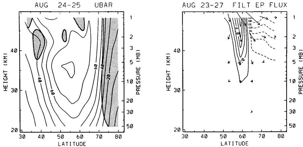
FIG. 12. (left) Zonal-mean zonal wind for 24–25 August. Heavy contours with shading denote \bar{q}_y < 0 . (right) EP flux diagram for the 4-day wave (filtered data) averaged over 23–27 August. Contours are 1 \text{ m s}^{-1}/\text{day} , and zero contours are omitted.
