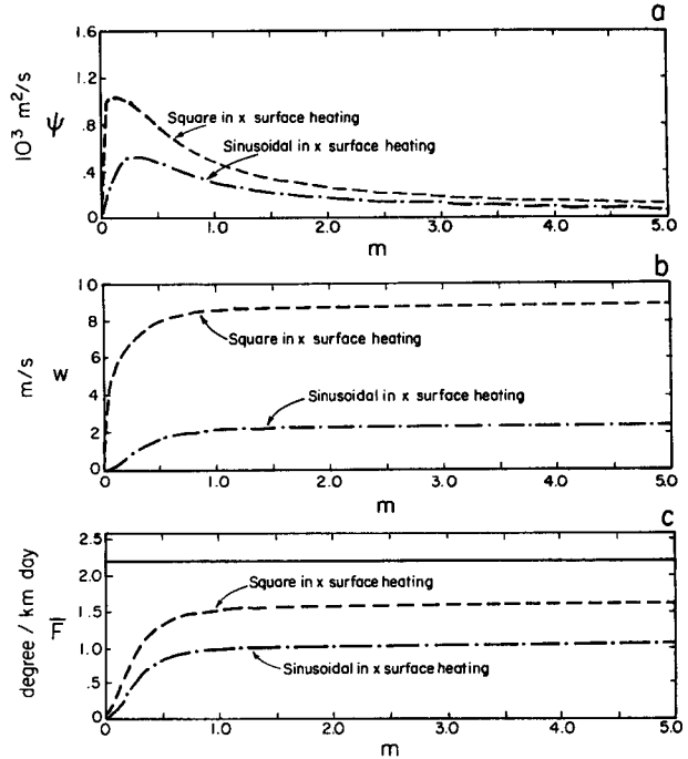
FIG. 4. (a) Intensity of the flow \psi_{0m} induced by a sinusoidal (dash-dotted line) and by a square periodic forcing (dashed line) versus horizontal wavenumber m . (b) Vertical velocity w_{0m} for a sinusoidal (dash-dotted line) and for a square periodic forcing (dashed line). (c) Flux intensities at z = 500 \text{ [m]} ; diabatic heat flux \bar{F}_D (solid line); mesoscale heat flux \bar{F}_{M\theta} for a sinusoidal (dash-dotted line) and for a square periodic forcing (dashed line).
