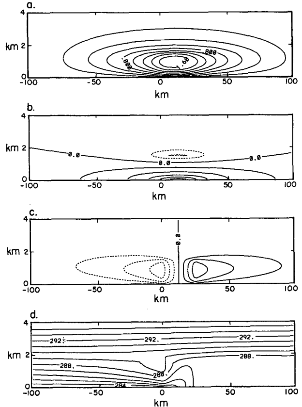
FIG. 1. Sea-breeze flow in a mature state. (a) Streamfunction \psi , \Delta\psi = 0.2 [ 10^3 \text{ m}^2 \text{ s}^{-1} ], 40^\circ of latitude ( \lambda = \omega ), h_0 = 1500 \text{ m} , R_0 = 100 \text{ km} . (b) Horizontal momentum component u , \Delta u = 1 [ \text{m s}^{-1} ]. (c) Vertical momentum component w , \Delta w = 1 [ \text{cm s}^{-1} ]. (d) Potential temperature \theta , \Delta\theta = 1 [K].
