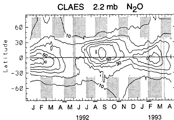
FIG. 4. Latitude–time variation of zonal-mean N_2O (ppbv) at 2.2 mb obtained from CLAES measurements. Shaded regions denote periods where CLAES data are unavailable.
