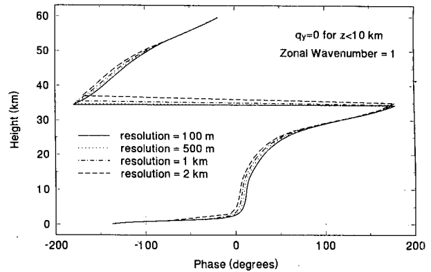
FIG. 15. Amplitude (a) and phase (b) of geopotential response to stationary forcing as a function of z for s = 1 , a fully adjusted basic state, and various resolutions.
