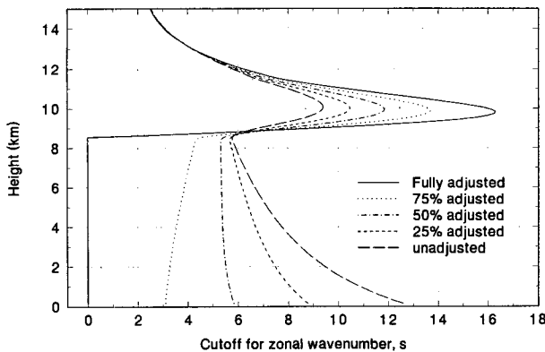
FIG. 16. Plot of s_{\text{cutoff}} as a function of z for various degrees of adjustment. See text for details.
