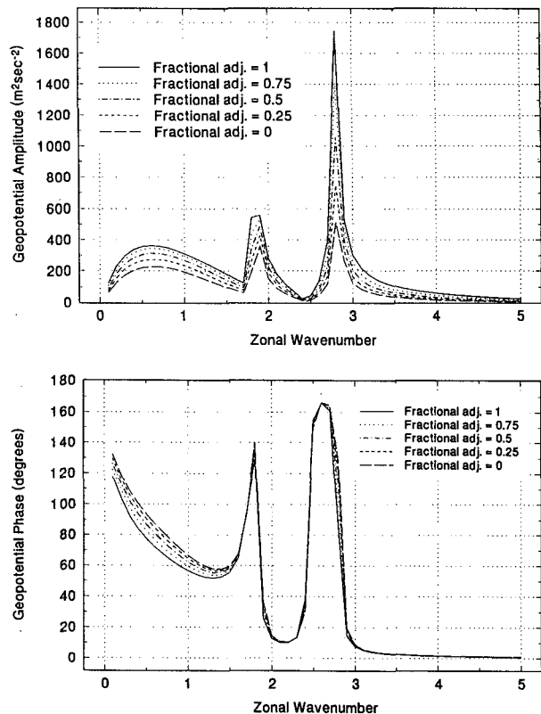
FIG. 5. Same as Fig. 3 but for response at 25 km.
