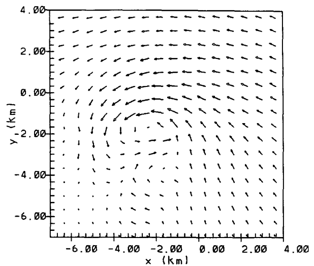
FIG. 8. Horizontal cross section of the horizontal storm-relative wind vectors at 1095 m and 95 min into the simulation. The maximum wind vector is 28.0 \text{ m s}^{-1} .
