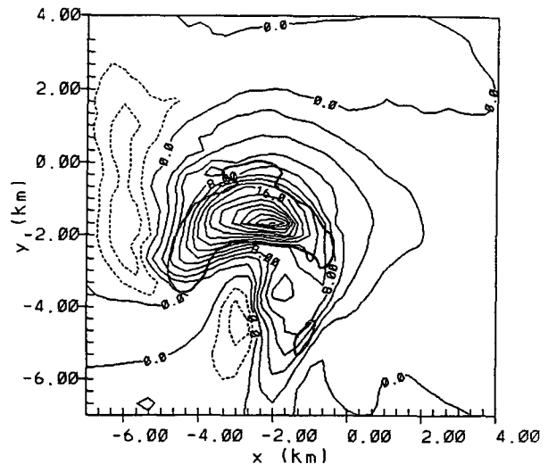
FIG. 7. Horizontal cross section of vertical motion at 1095 m and 95 min into the simulation. The contour interval is 2.0 \text{ m s}^{-1} . The maximum upward motion is 30.0 \text{ m s}^{-1} and the maximum downward is -4.0 \text{ m s}^{-1} . The dark solid depicts the boundary, vertical vorticity of 0.01 \text{ s}^{-1} for the mesocyclone.
