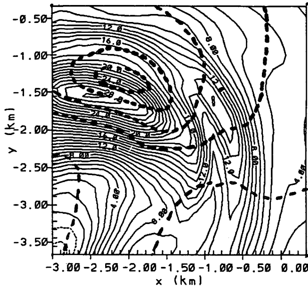
FIG. 11. Horizontal cross section at 1095 m and 94 min into the simulation. Solid contours depict upward motion contoured at 1 \text{ m s}^{-1} and the bold dashed contours depict the perturbation pressure. The maximum updraft is 29 \text{ m s}^{-1} . The contours for the pressure field are -120, -240, -360, -480, and -540 \text{ Pa} .
