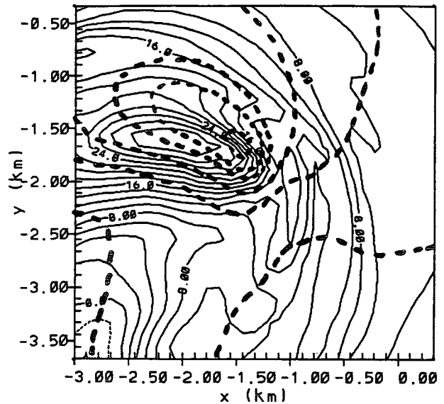
FIG. 12. Same as Fig. 11 at 95 min. The contours for the pressure field are -120, -240, -360, -480, -510, and -660 \text{ Pa} .
