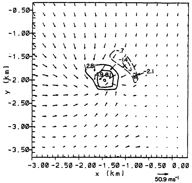
FIG. 26. Same as Fig. 20 except at 11 m.
