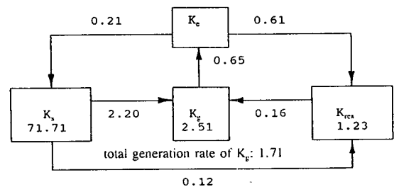
FIG. 5. Kinetic energy budgets for cases C_1 , C_0 , and C_2 at hour 48. The values in boxes denote the energy in units of 10^{12} \text{ m}^4 \text{ s}^{-2} , and the other values represent the energy conversions in units of 10^7 \text{ m}^4 \text{ s}^{-3} . The arrows indicate direction of energy transfer.
