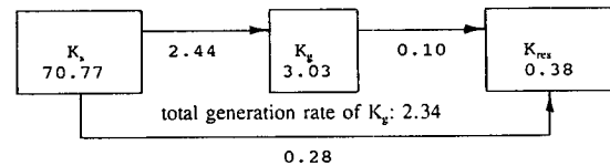
(c) Case C_2 (Constant cyclonic meridional shear)
