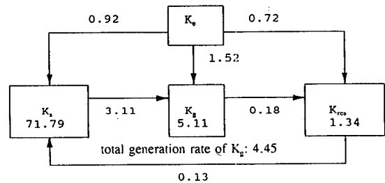
(b) Case C_0 (Resting environment)
