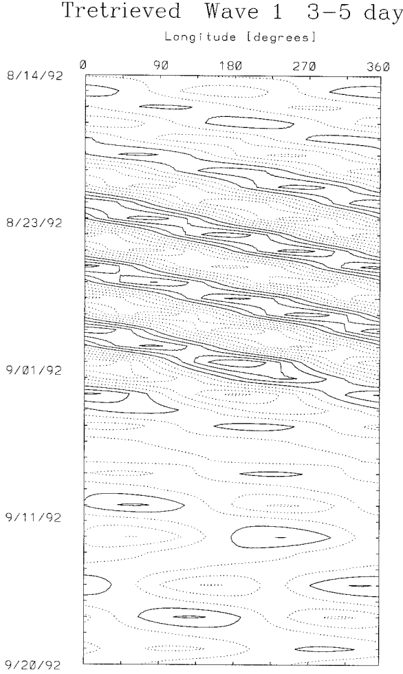
FIG. 2. Time vs longitude plot of T_{\text{retrieved}} at 64^{\circ}\text{S} and 1 hPa (48 km) filtered for wave 1 and 3–5 day periods (eastward and westward) for 14 August–20 September 1992. Dashed contours are from -4 to 0 K by 1 K. Solid contours are from 1 to 4 K by 1 K.
