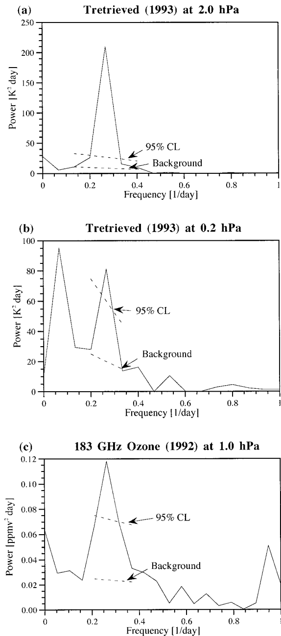
FIG. 9. Unsmoothed power spectra for wave 1 at 72^{\circ}\text{S} plotted along with estimated background and 95% confidence level. (a) T_{\text{retrieved}} for the 1993 series at 2 hPa. (b) T_{\text{retrieved}} for the 1993 series at 0.2 hPa. (c) 183-GHz ozone for the 1992 series at 1.0 hPa.
