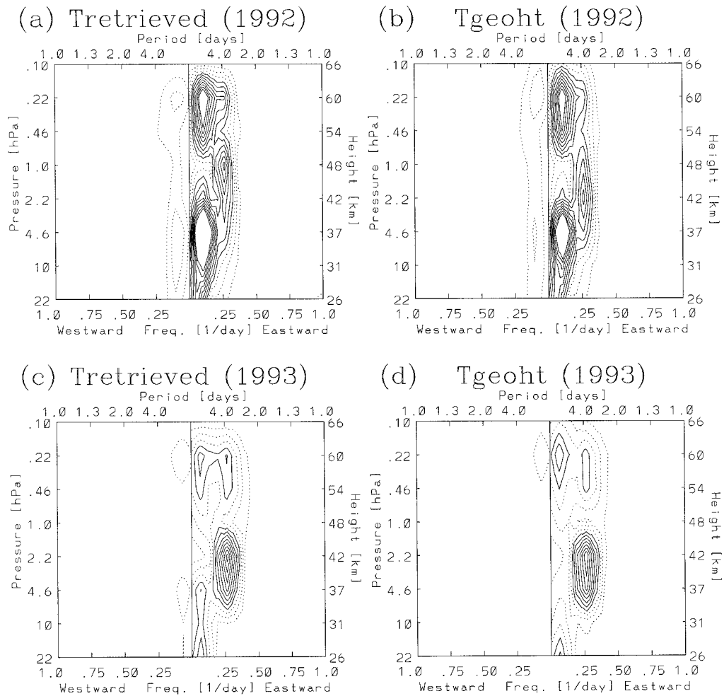
FIG. 1. (a) East–west power spectrum for wave 1 MLS temperature ( T_{\text{retrieved}} ) at 72^{\circ}\text{S} for 18 August–6 September 1992. Dashed contours are at 10, 20, and 30 \text{K}^2 \text{ day} , and solid contours are from 40 to 100 \text{K}^2 \text{ day} by 10 \text{K}^2 \text{ day} . (b) Same as (a) but for temperature derived from MLS geopotential height ( T_{\text{geoht}} ). (c),(d) Same as (a),(b) but for 2–16 September 1993.
