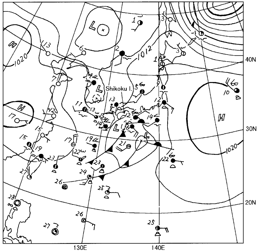
FIG. 5. Synoptic chart at 1200 UTC 11 April 1995. Surface wind vectors full barb = 5 \text{ m s}^{-1} ; half-barb = 2.5 \text{ m s}^{-1} . Cloud cover (octants) are shown within station circle.
