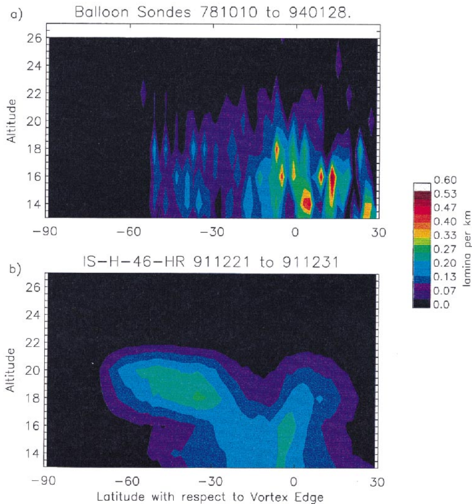
FIG. 5. Lamina frequencies as a function of altitude and the latitudinal distance from the vortex edge: (a) from Dec–Jan climatology of the balloon sondes from 1978 to 1994, vs (b) from 1^\circ latitude by 1.25^\circ longitude isentropic model IS-H-46-HR during the last 10 days of the integration. The units of lamina frequencies are the number of laminar events per km in the vertical.
