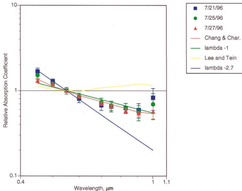
FIG. 4. Normalized aerosol absorption coefficients as a function of wavelength. Also shown is a \lambda^{-1} curve and calculations using Eq. (1) with the Lee and Tein, and Chang and Charalampopoulos refractive indices. The chi-squared value for the Chang and Charalampopoulos refractive indices is 0.79 (rms error 0.085), 1.97 for the constant refractive index (rms error 0.12), and 38.23 for the Lee and Tien refractive indices (rms error 0.49).
