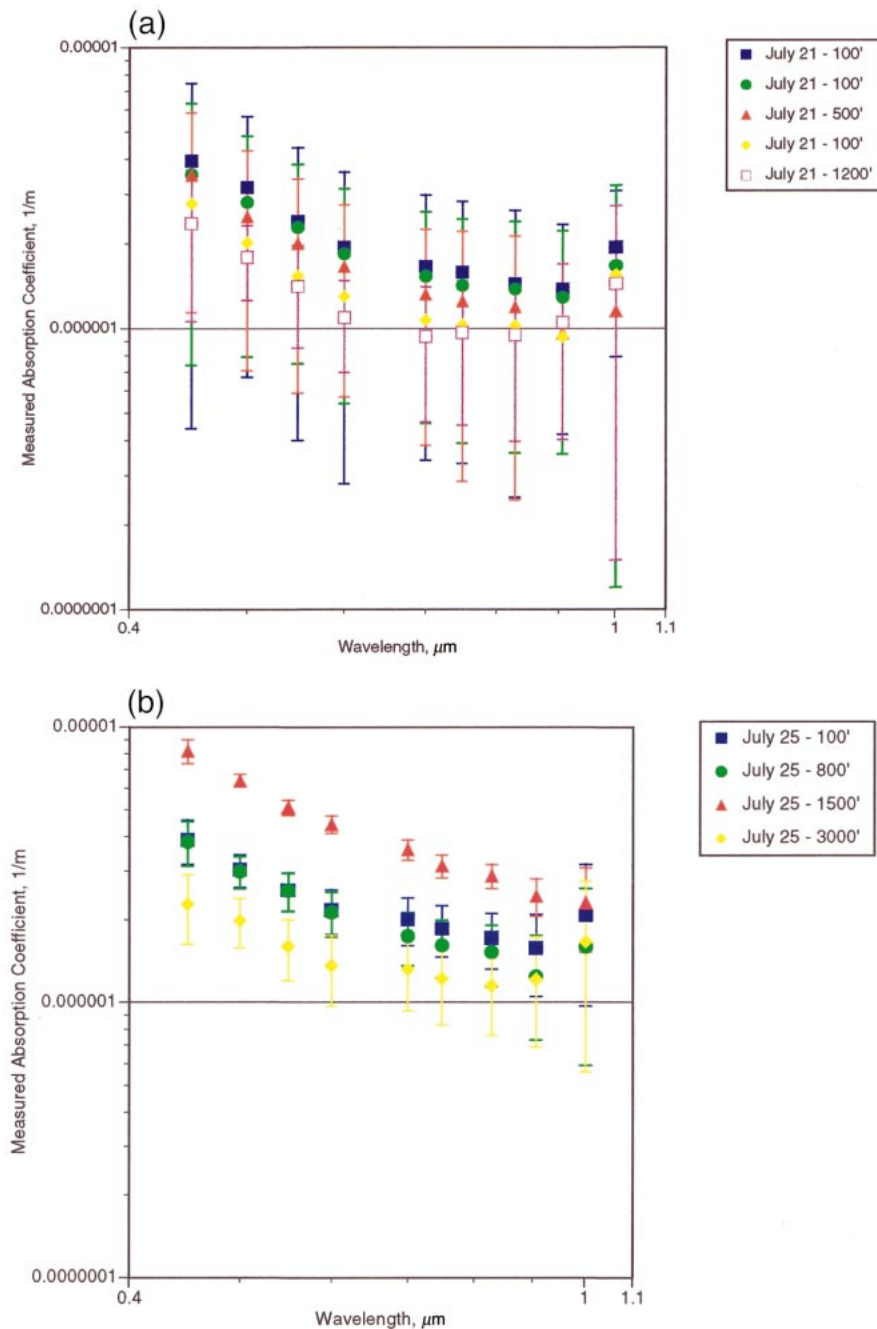
FIG. 1. Aerosol absorption coefficients as a function of wavelength for three TARFOX days: (a) 21, (b) 25, and (c) 27 July.
