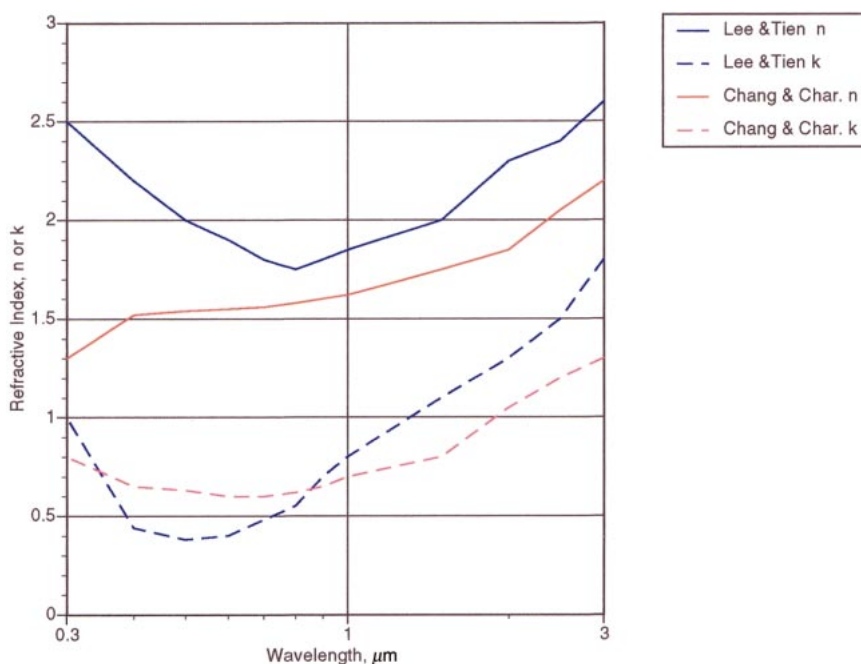
FIG. 3. Refractive indices for flame soots from Lee and Tien (1981) and Chang and Charalampopoulos (1990).
