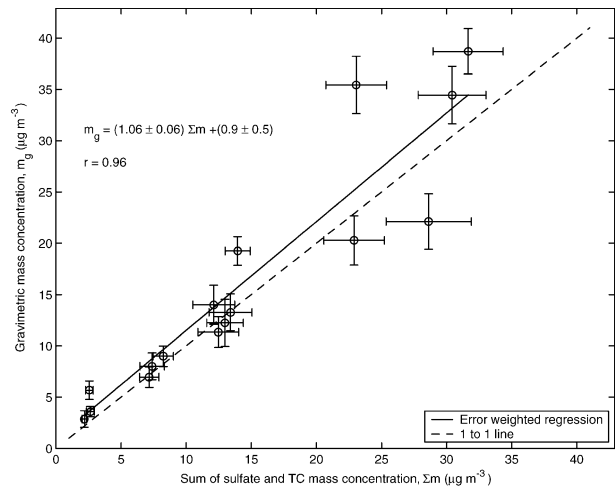
FIG. 5. Error-weighted linear regression of the gravimetric mass concentration m_g to the sum of the sulfate and total carbon species mass concentrations \Sigma m . The equation for the error-weighted regression line (solid line) is given on the graph. The dashed line is the 1-to-1 perfect correlation line. Error bars are the uncertainty in m_g and the propagation of the uncertainty in \Sigma m , all of which are listed in Table 4.
