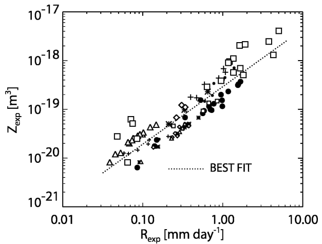
FIG. 11. (a) Derived reflectivities Z_{\text{exp}} plotted against precipitation rates R_{\text{exp}} for all the in-cloud extrapolated distributions. The dotted line represents the best fit power law with parameters given in Table 2. Symbols as for Fig. 10.
