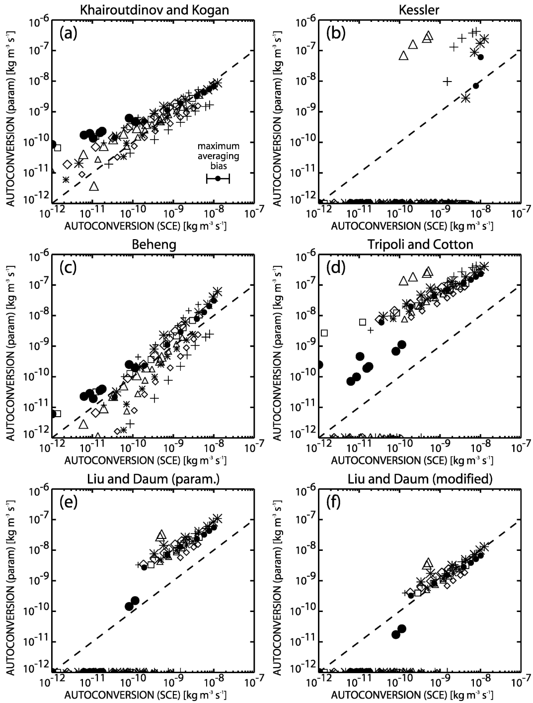
FIG. 4. Comparison of autoconversion rates derived from the SCE and observed DSDs (abscissas) and from the bulk parameterizations of (a) Khairoutdinov and Kogan (2000); (b) Kessler (1969); (c) Beheng (1994); (d) Tripoli and Cotton (1980); (e) Liu and Daum (2004); and (f) modified Liu and Daum (2004). Formulations for the parameterized autoconversion rates are presented in Table 1. Points for which the parameterized autoconversion rates are zero are shown along the abscissas. The symbols are shown in Fig. 6. The estimated maximum bias in each direction caused by using a layer mean DSD is also shown.
