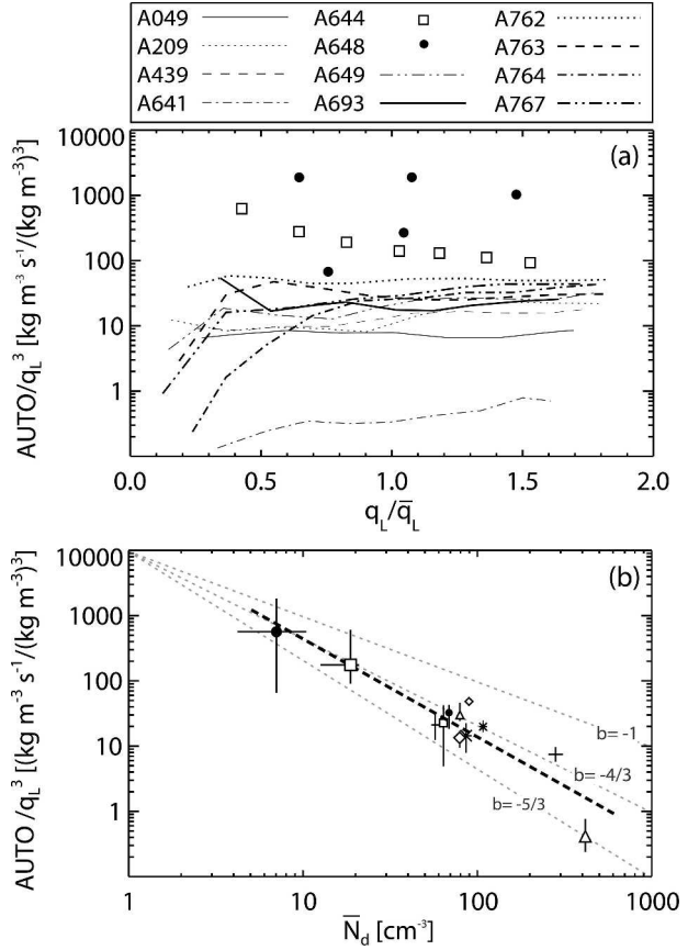
FIG. 5. (a) SCE-derived autoconversion rates normalized with q_L^a ( a = 3 ) to best remove systematic dependence upon liquid water content. Line and symbol types shown above the plot. (b) Normalized autoconversion rates plotted against mean cloud droplet concentration. Symbols are those shown in Fig. 4. Light dashed lines show the power laws with b = -1 , -4/3 , and -5/3 . Heavy dashed line shows best fit from the residual analysis (see text).
