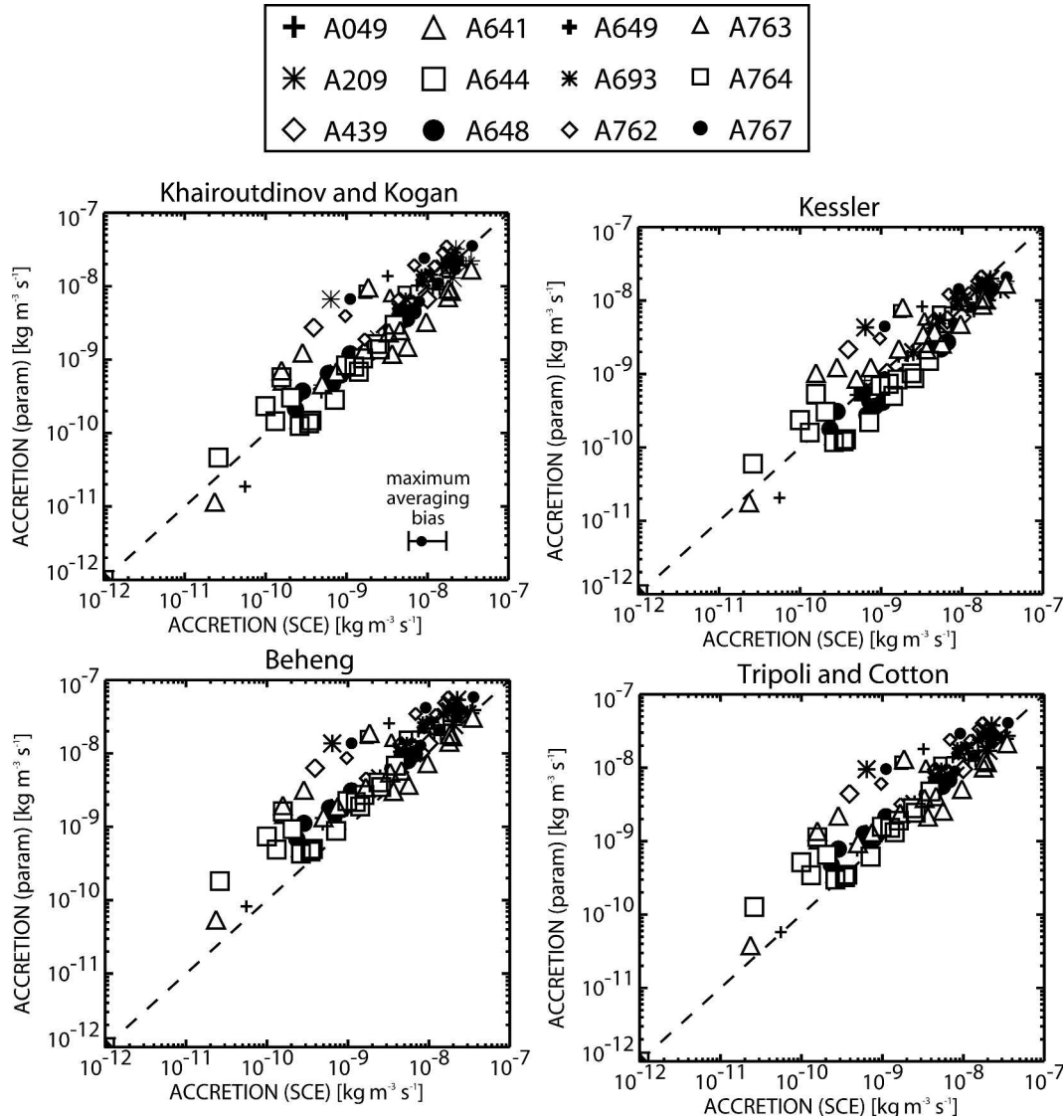
FIG. 6. As for Fig. 4 but comparing accretion parameterizations.
