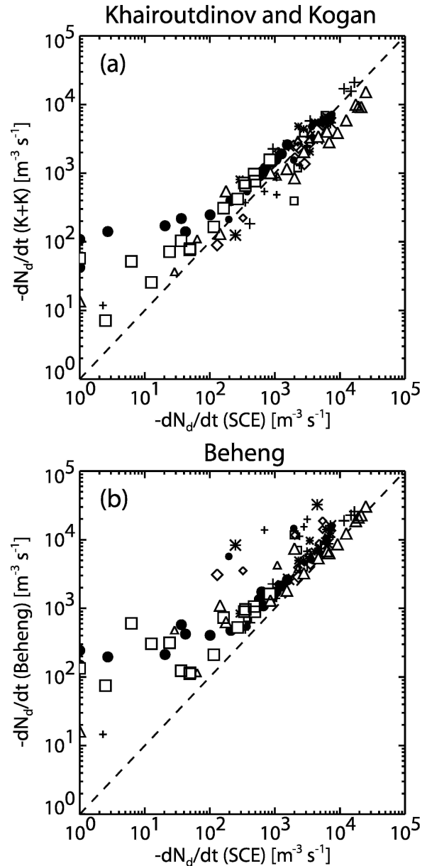
FIG. 7. Comparison of combined autoconversion/accretion rate of loss of cloud droplets derived from the observed droplet size distributions (abscissa) with those parameterized (ordinate) assuming that all collected drops have the size of the mean volume radius of the cloud drops r_v .
