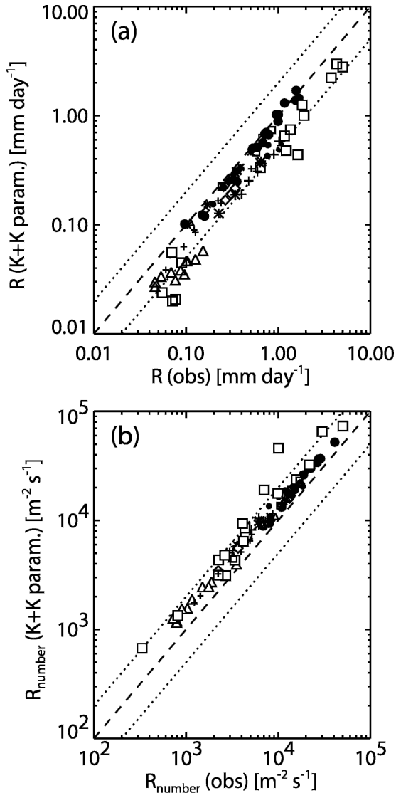
FIG. 8. (a) Mass and (b) number of fall rates as defined in Eqs. (8) and (9) compared with those using the parameterization of Khairoutdinov and Kogan (2000). Dashed lines show perfect agreement; dotted lines show factor of 2 errors.
