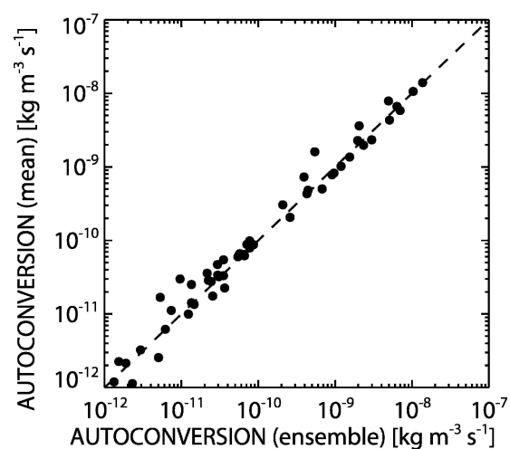
FIG. A1. Comparison of autoconversion rate derived from the ensemble DSD for entire 20–60-km straight and level runs (abscissa), against the mean of the autoconversion rates calculated for each 1-km subsection of the run.
