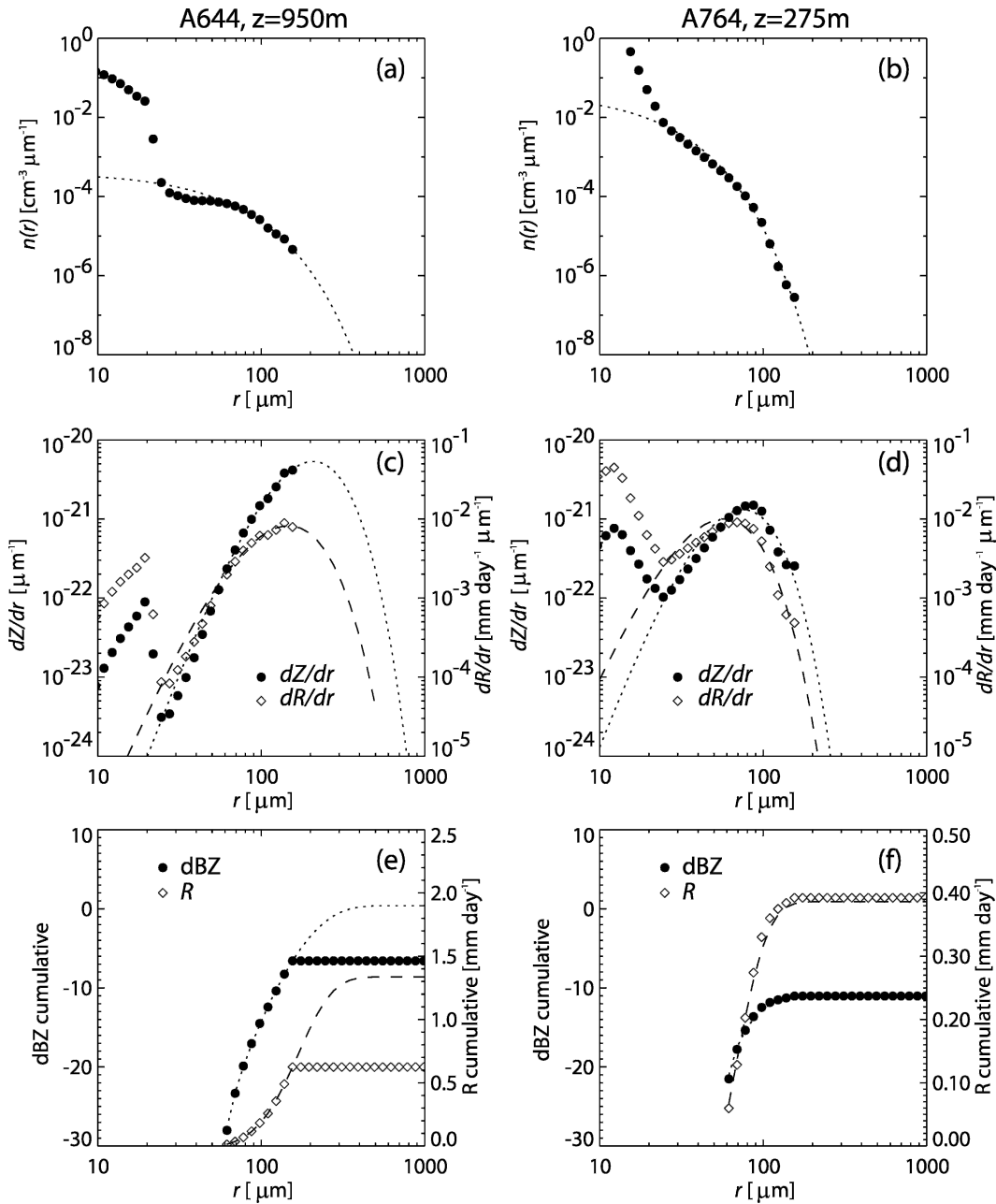
FIG. 3. Examples from two flights showing (a), (b) drop size distributions, (c), (d) size-resolved radar reflectivity dZ/dr and precipitation rate distributions dR/dr , and (e), (f) the cumulative values of dBZ integrated from r = 60 \mu\text{m} upward. Data values obtained using the 2D-C and FSSP probes are shown using symbols, and dashed and dotted lines show the fitted exponential distributions. For the z = 950 \text{ m} run in flight A644 (left), the exponential distribution suggests that both Z and R have contributions from drops larger than those actually measured. For the z = 275 \text{ m} run in A764 the measurements capture almost entirely the contributions to Z and R .
