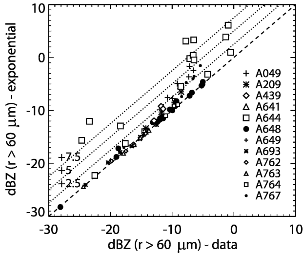
FIG. 10. Reflectivity factor dBZ derived using droplets with radii larger than 60 \mu\text{m} for data values (abscissa) and for the fitted exponential distributions extrapolated to r = \infty (ordinate). In most cases there is only a small difference between the two values, indicating that the 2D-C sample volume is sufficiently large enough to account for significant contributions to reflectivity from all droplet sizes. However, in A644 there are differences of at least 10 dBZ in some cases, which arise because drops larger than those measured using the 2D-C are contributing significantly to the reflectivity.
