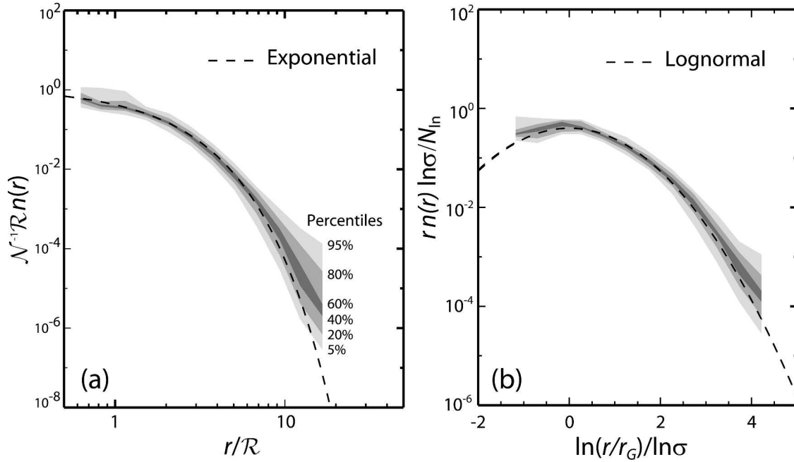
FIG. 2. (a) Normalized DDSDs (\mathcal{R}/\mathcal{N})n(r) at all in-cloud levels (103 spectra) plotted against r/\mathcal{R} . The universal exponential distribution n_{\text{exp}}(r) = (\mathcal{R}/\mathcal{N})n(r) = \exp(-r/\mathcal{R}) is shown by the dashed line. The spectra are shown by contours that denote percentiles of all the distributions in each r/\mathcal{R} class. The lightest colored contour therefore contains 95% of all the DDSD in each class. (b) As in (a) but normalized DDSDs [rn(r) \ln\sigma/N_{\text{in}}] plotted against \ln(r/r_G)/\ln\sigma . The universal lognormal distribution n_{\text{ln}}(r) = rn(r) \ln\sigma/N_{\text{in}} = (1/\sqrt{2\pi}) \exp[-\ln^2(r/r_G)/2 \ln^2\sigma] is shown by the dashed line. See text for the definition of the parameters.
