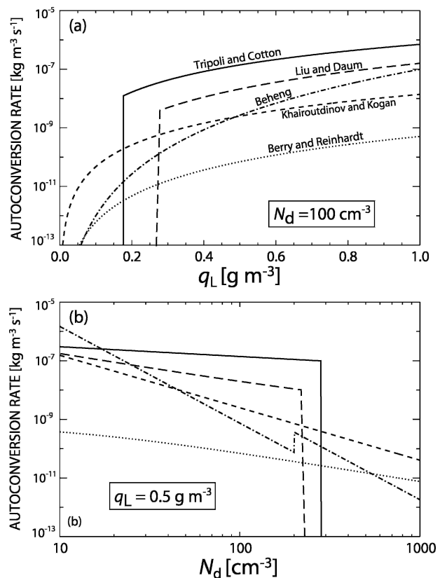
FIG. 1. Comparison of parameterized autoconversion rates from widely used schemes [all except the Berry and Reinhardt scheme (Berry and Reinhardt 1974), which is not examined further in this paper, are defined in Table 1]. (a) Autoconversion rate as a function of liquid water content for a fixed cloud droplet concentration of N_d = 100 \text{ cm}^{-3} . (b) Autoconversion rates as a function of droplet concentration for a fixed liquid water content of q_L = 0.5 \text{ g m}^{-3} .
