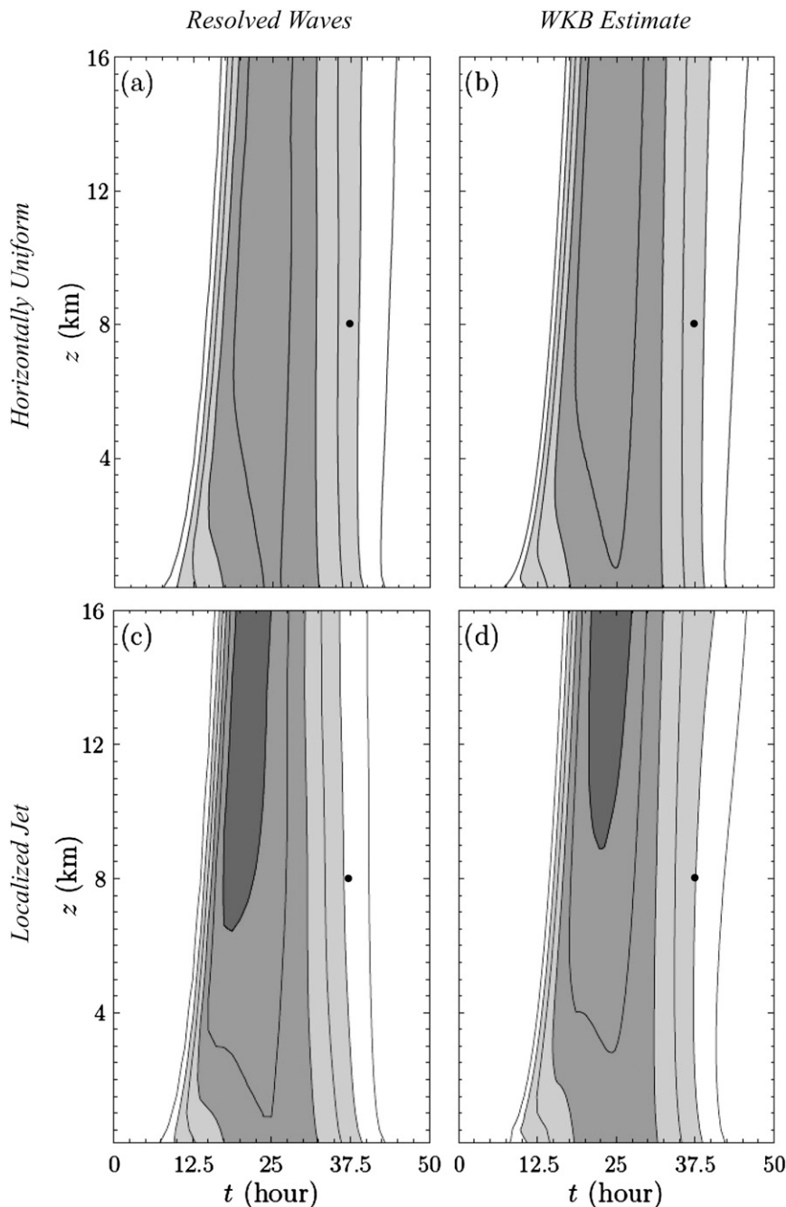
FIG. 1. Gravity wave momentum flux integrated over the horizontal domain as a function of t and z for (a),(b) the horizontally uniform flow and (c),(d) the barotropic jet. The direct evaluation of the fluxes due to gravity waves resolved in the numerical model is presented in (a) and (c); (b) and (d) show the fluxes computed using ray-tracing theory and conservation of wave action. The contour interval is 10^8 N; steps in the gray shading are at -2 \times 10^8 , -4 \times 10^8 , and -6 \times 10^8 N.
