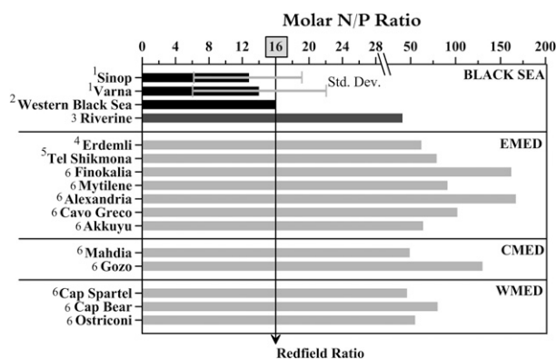
FIG. 6. DIN:DIP molar ratios for the present study and from the literature for the Black Sea: 1) current study, 2) Medinets and Medinets (2012), and 3) Ludwig et al. (2009); and for the Mediterranean Sea: 4) Koçak et al. (2010), 5) Herut et al. (1999, 2002), and 6) Markaki et al. (2010).
