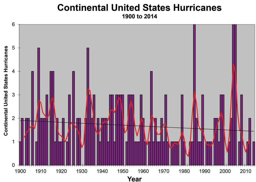
FIG 1. Continental U.S. hurricanes from 1900 through 2014. The time series is derived from the updated format of the Atlantic hurricane database (HURDAT2; Landsea and Franklin 2013) with results from the reanalysis (Landsea et al. 2008, 2012, 2014; Hagen et al. 2012) incorporated through 1955. The red curve provides a 1–2–1 filter applied twice to smooth interannual variability. The black line provides the linear trend.
