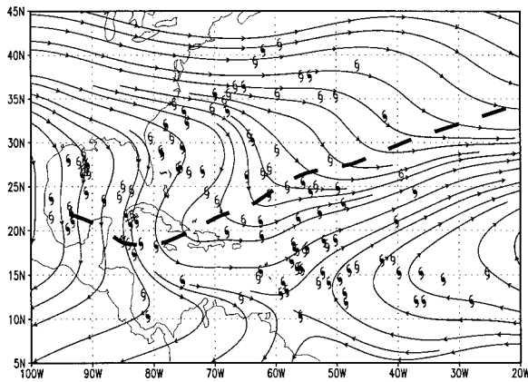
FIG. 14. Diagram depicting where TCs were first named hurricanes during the 10 yr with the highest (tropical storm symbols), and the ten lowest (hurricane symbols) SLP anomalies in TA along with the climatological TUTT axis during JAS.
