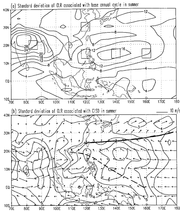
FIG. 3. (a) Standard deviation of the base annual cycle of OLR ( \text{W m}^{-2} ) in northern summer from May to October. The five boxes indicate the locations for which CISO OLR are shown in Fig. 6. (b) Same as in (a) except for the Climatological Intraseasonal Oscillation (CISO) component of OLR. Arrows show summer mean 850-hPa winds. Heavy solid and dashed lines outline the positions of subtropical ridge and monsoon trough, respectively.
