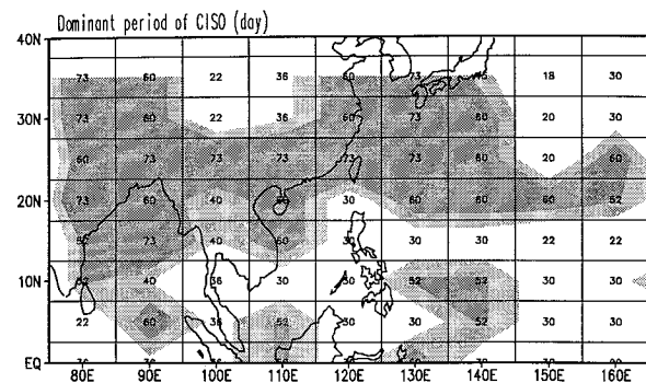
FIG. 4. Spatial variation of the dominant period of CISO in units of days. Dark and light shadings represent areas where CISO period is longer than 50 days and between 40 and 50 days, respectively.
