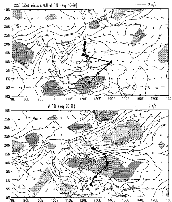
FIG. 11. The extremely wet (P28) (a) and dry (P30) (b) phases of CISO Cycle I. Contours show OLR anomalies at an interval of 3 \text{W m}^{-2} and arrows show anomalous 850-hPa winds. Heavy (light) shadings denote, respectively, areas with statistically significant wet (dry) singularity at 95% confidence level. The heavy triangle indicates the center of OLR anomalies at the extremely wet or dry phases. Heavy solids along with the arrows indicate the tracks of the OLR anomaly centers on consecutive pentad maps.
