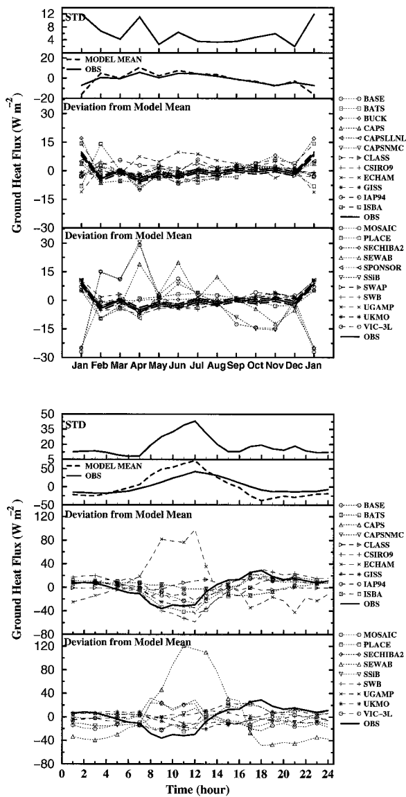
FIG. 8. As in Fig. 3 except for ground heat flux ( \text{W m}^{-2} ). The two thick dashed lines in panels 3 and 4 represent the estimated \pm 1 \text{ W m}^{-2} observation errors.
