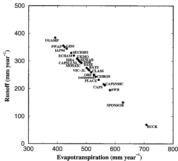
FIG. 10. Annual runoff versus evapotranspiration (mm yr -1 ).
