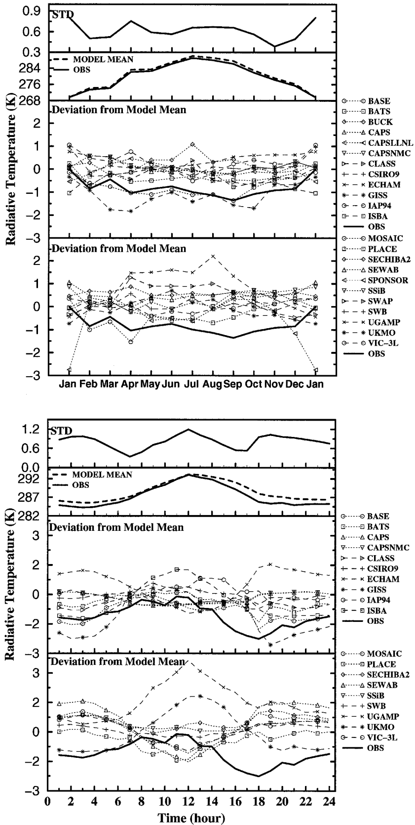
FIG. 4. As in Fig. 3 except for surface radiative temperature (K).
