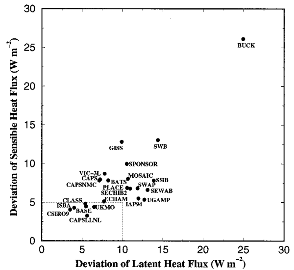
FIG. 9. Averaged rms deviation from monthly observation for sensible versus latent heat fluxes ( \text{W m}^{-2} ).
