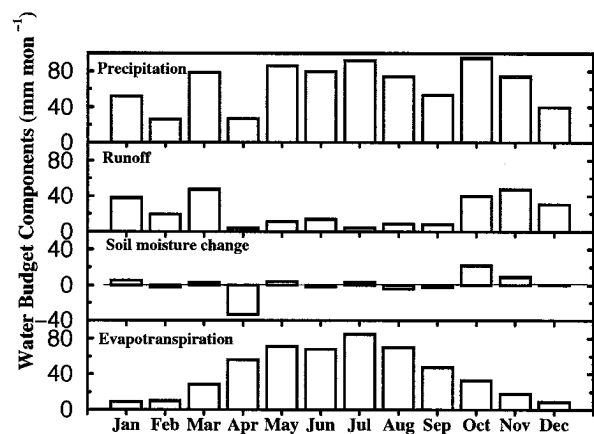
FIG. 11. Model mean (except precipitation) monthly water balance components (mm month -1 ).
